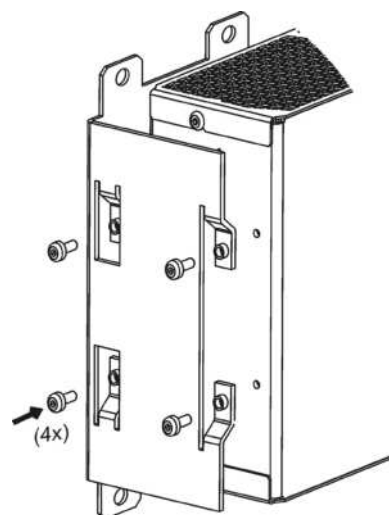
Fig. 3-3 Mounting steel bracket
