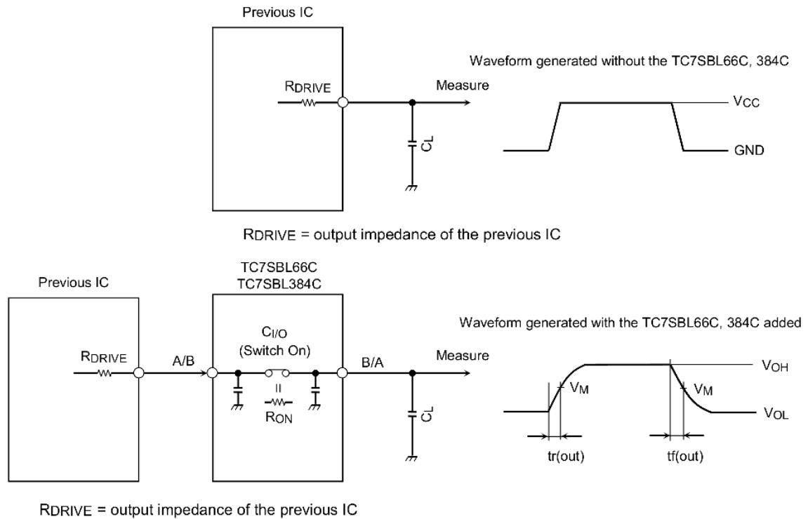
Fig. 12.1 Calculation Circuit
