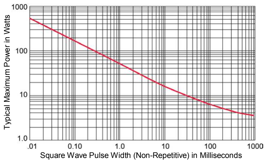
FIGURE 2 TRANSIENT SURGE CAPABILITY
