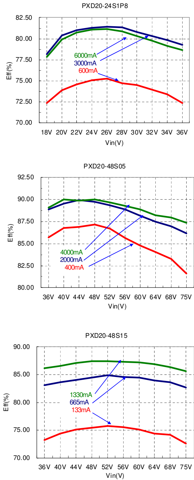
b. Efficiency with line change under different load conditions at room temperature
