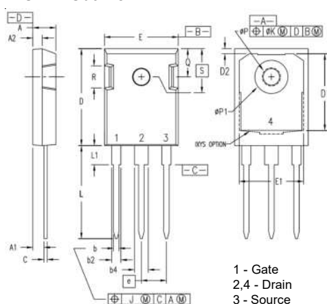
TO-247 Outline
