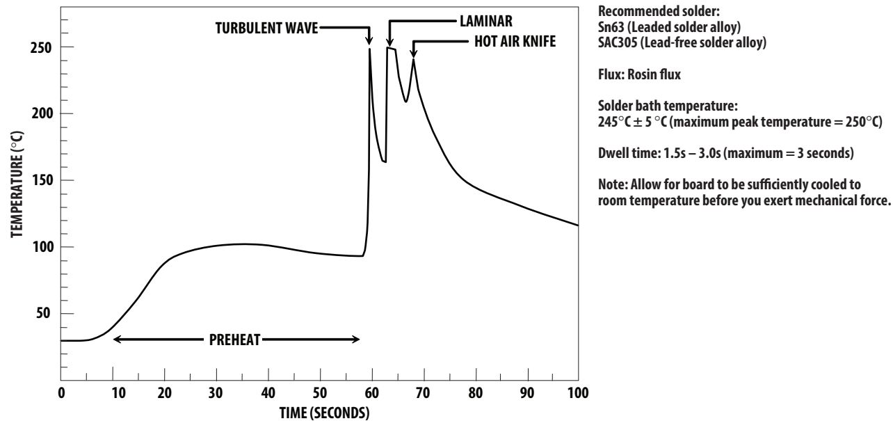
Figure 14: Example of Wave Soldering Temperature Profile for TH LED
