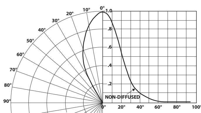
Figure 13: Relative Luminous Intensity vs. Angular Displacement
