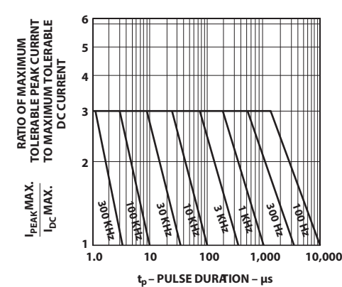
Figure 8: Maximum Tolerable Peak Current vs. Pulse Duration ( I_{DCMAX} as per MAX Ratings)
