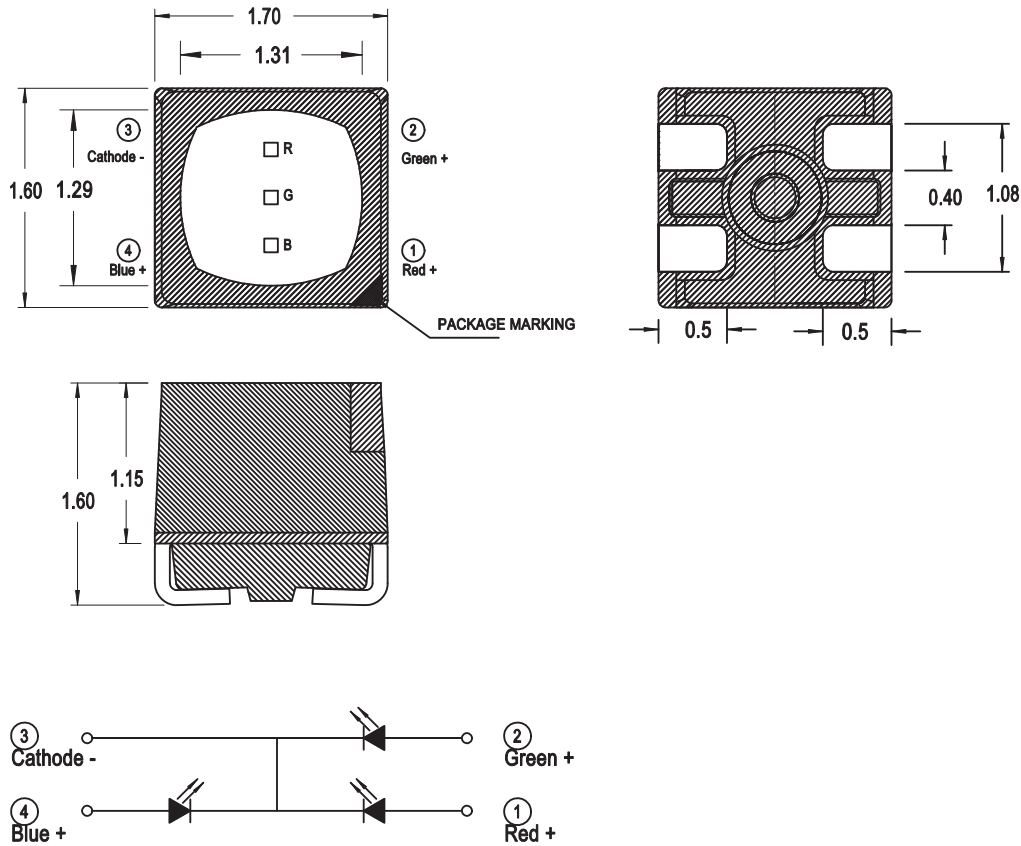
Figure 2: Package Drawing
