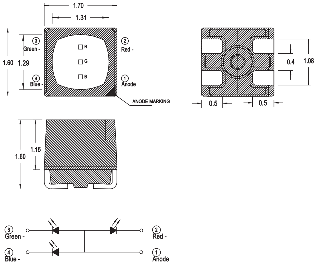
Figure 1: Package Drawing
