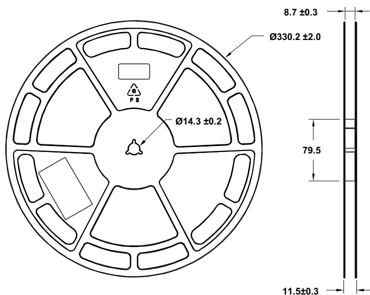
Figure 15: Reel Drawing
