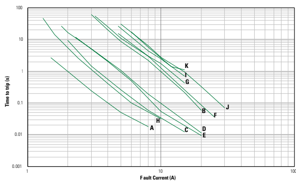
Typical Time-to-Trip Curves at 25°C Automotive Terminal SMD Series
