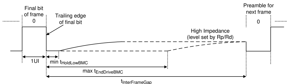
Figure 3. t_{InterFrameGap}
