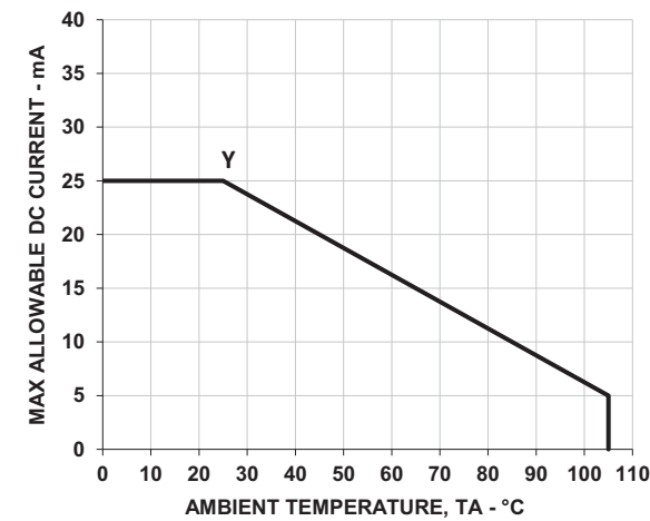
Figure 7: Allowable DC Current vs. Ambient Temperature
