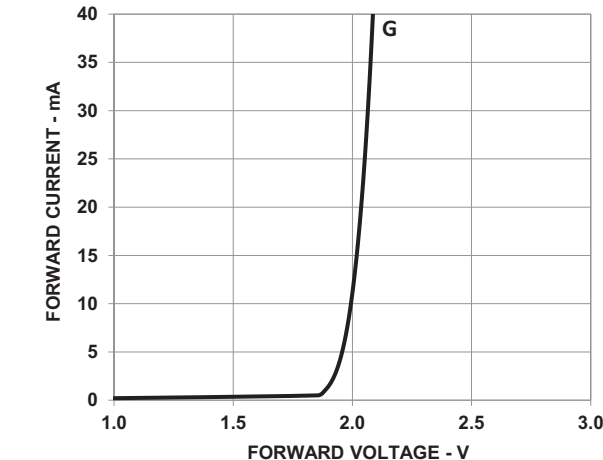
Figure 4: Forward Current vs. Forward Voltage
