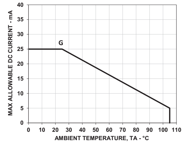
Figure 3: Allowable DC Current vs. Ambient Temperature
