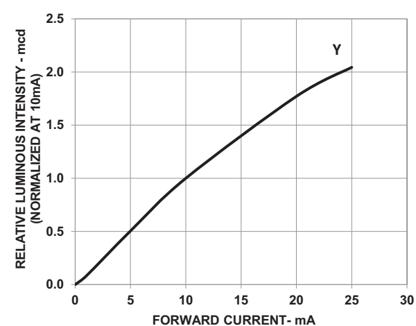
Figure 6: Relative Intensity vs. Forward Current
