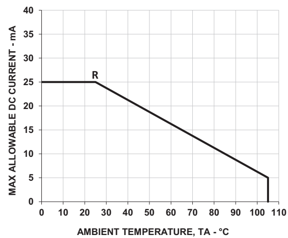
Figure 11: Allowable DC Current vs. Ambient Temperature
