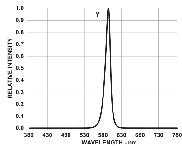
Figure 5: Relative Intensity vs. Wavelength
