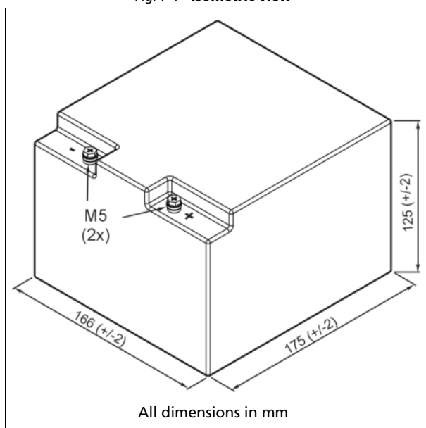
Fig. 7-1 Isometric view
