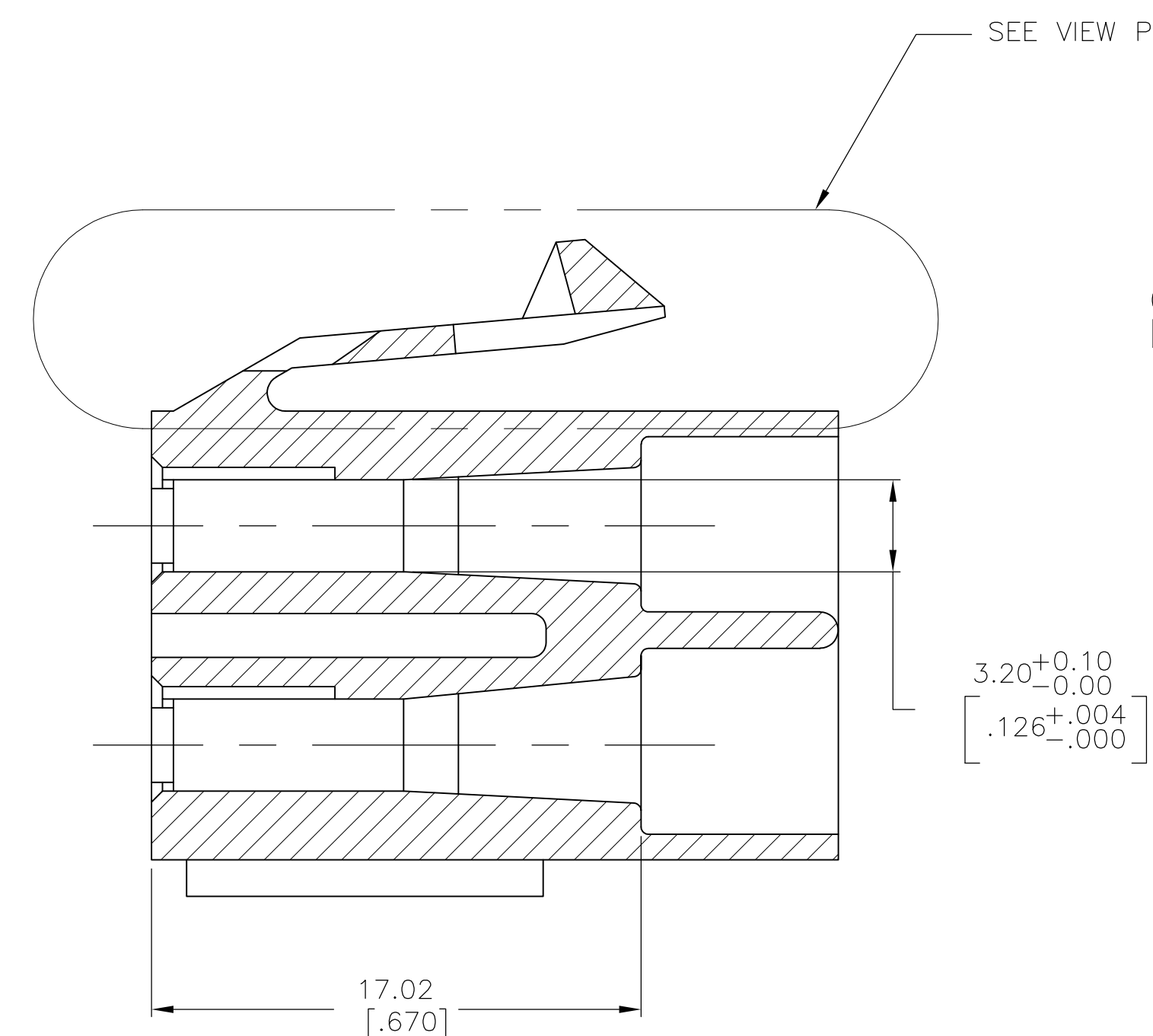
SECTION R-R
