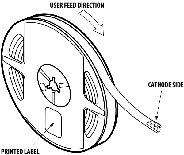
Figure 28: Reeling Orientation
