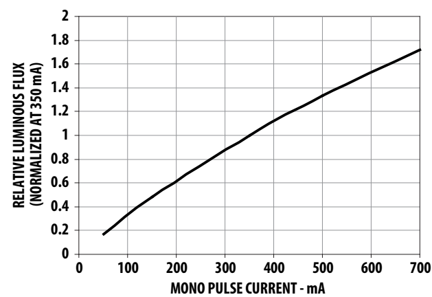
Figure 13: Relative Luminous Flux vs. Mono Pulse Current
