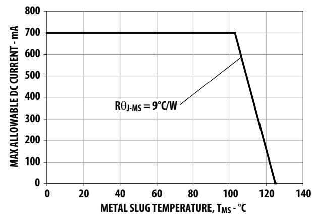
Figure 11: Maximum Forward Current vs. Ambient Temperature. Derated based on T_{JMAX} = 125^{\circ}C , R\theta_{J-MS} = 9^{\circ}C/W .
