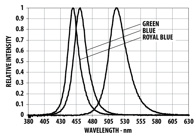
Figure 12: Relative Intensity vs. Wavelength for Royal Blue, Blue, and Green
