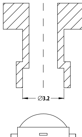
Figure 24: Recommended Pick-and-Pick Nozzle Tip. Inner diameter = 3.2 mm.
