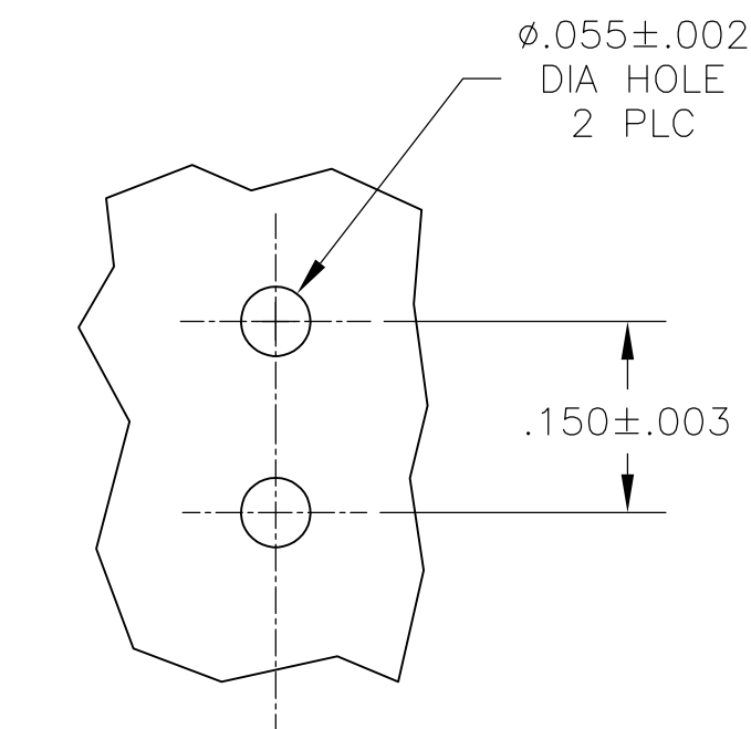
P.C. BOARD HOLES
