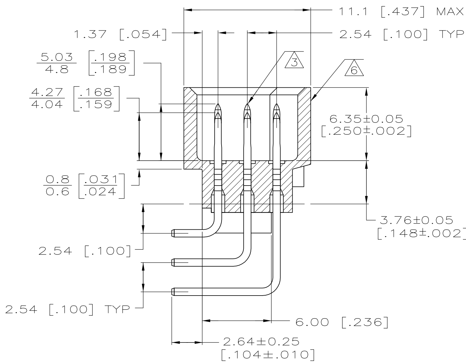
SECTION Z-Z
