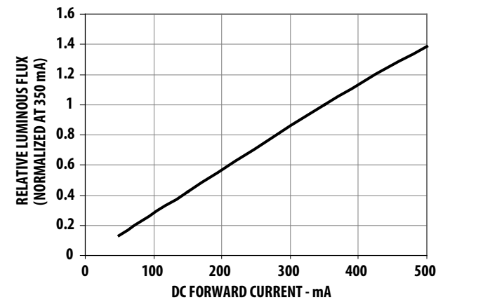
Figure 5: Relative Luminous Flux vs. Mono Pulse Current
