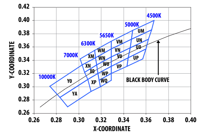
Figure 2: Color Bin Structure for Cool White
