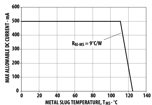
Figure 13: Maximum Forward Current vs. Metal Slug Temperature. Derated based on T_{JMAX} = 125^{\circ}C , R_{\theta J-MS} = 9^{\circ}C/W .
