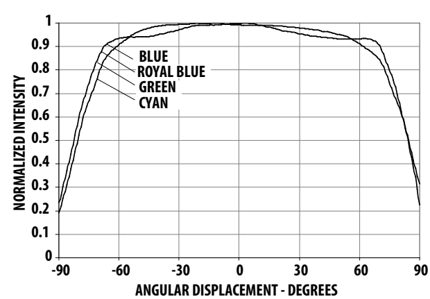
Figure 18: Radiation Pattern for Blue, Royal Blue, Cyan, and Green
