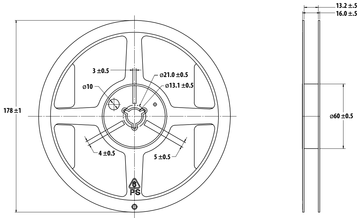
Figure 30: Reel Dimensions
