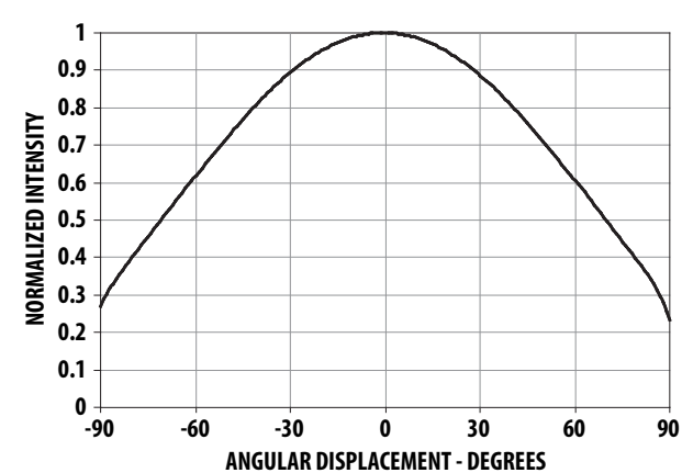
Figure 19: Radiation Pattern for Cool White and Neutral White
