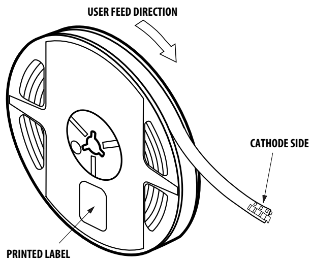
Figure 31: Reeling Orientation
