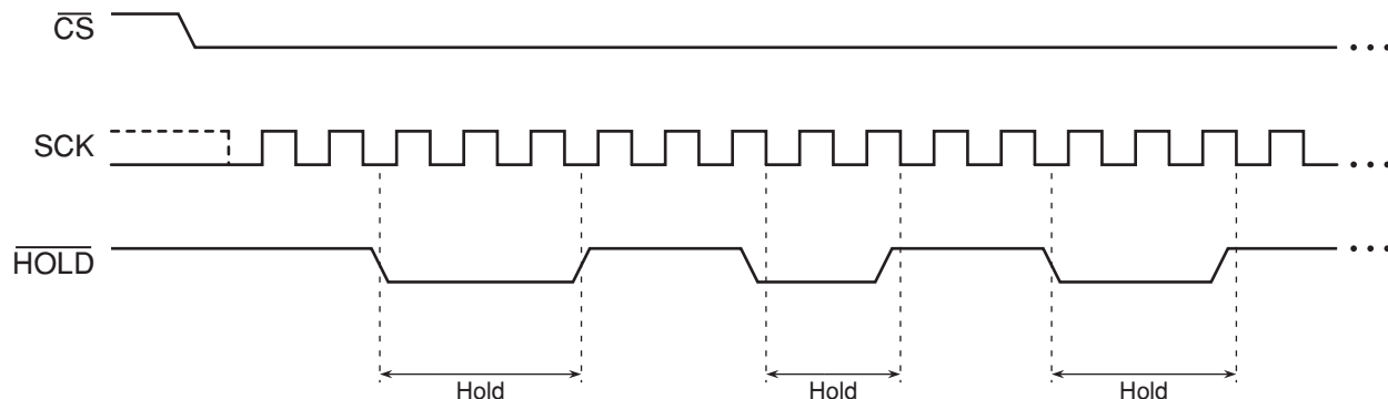
Figure 28. Hold Mode
