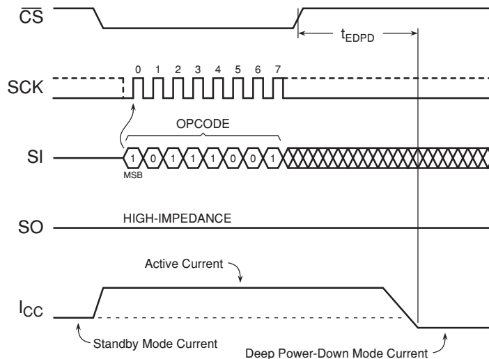
Figure 23. Deep Power-Down
