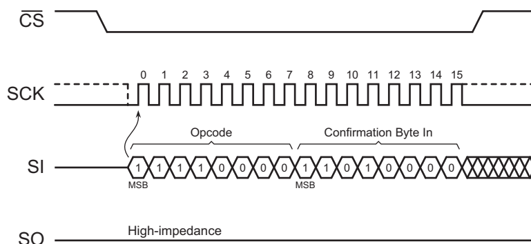
Figure 29. Reset
