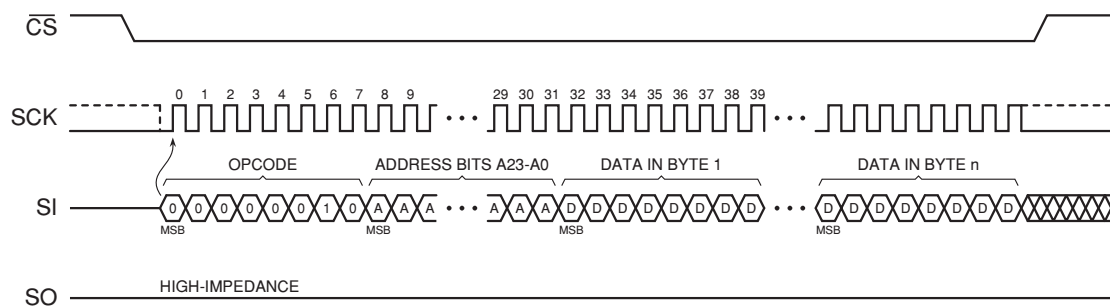
Figure 11. Page Program
