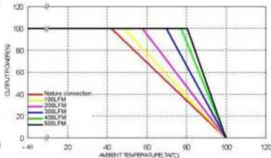
Derating Output Current Versus Ambient Temperature and Airflow Airflow V_{in} = V_{in(nom)}
