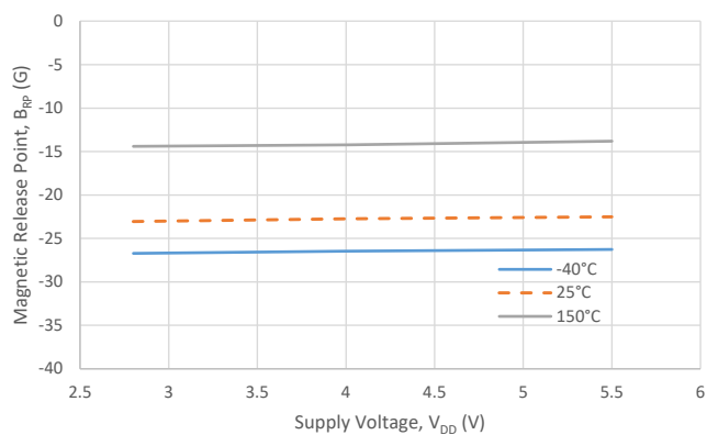
Release Point (B) vs. Supply Voltage
