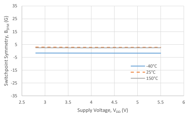
Symmetry (A) vs. Supply Voltage
