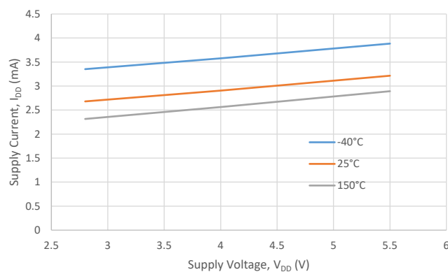
Supply Current (XY) vs. Supply Voltage
