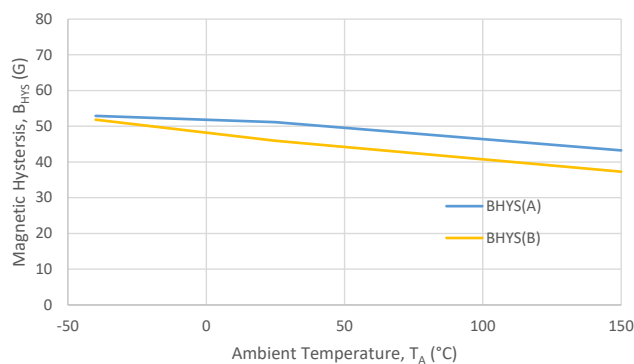
Hysteresis vs. Temperature
