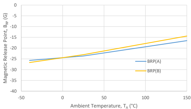
Release Point vs. Temperature
