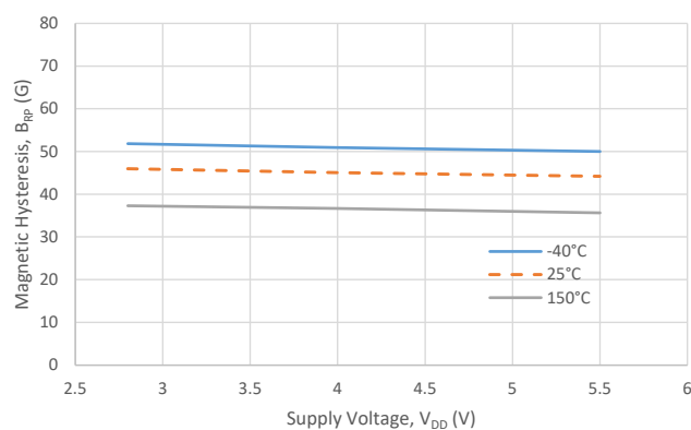
Hysteresis (B) vs. Supply Voltage
