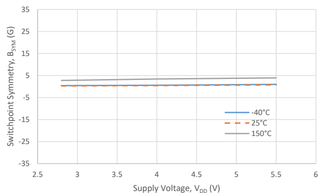
Symmetry (B) vs. Supply Voltage
