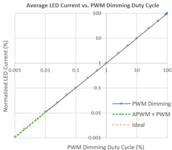
Figure 33: How to achieve 100,000:1 dimming ratio by using both PWM and APWM. Test conditions: V_{IN} = 12 V, V_{OUT} = 25 V ( 8 \times WLED), total LED current = 400 mA, PWM frequency = 200 Hz, APWM frequency = 100 kHz.
