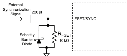
Figure 15: Countermeasure for External Sync Stuck-at-Low Fault
