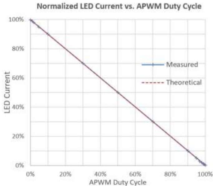
Figure 30: Showing LED current is inversely proportional to the APWM duty cycle. Test conditions: V_{IN}=12\text{ V} , V_{OUT}=25\text{ V} ( 8 \times \text{WLED} ), total LED current = 100\text{ mA} \times 4 , APWM frequency = 100\text{ kHz}
