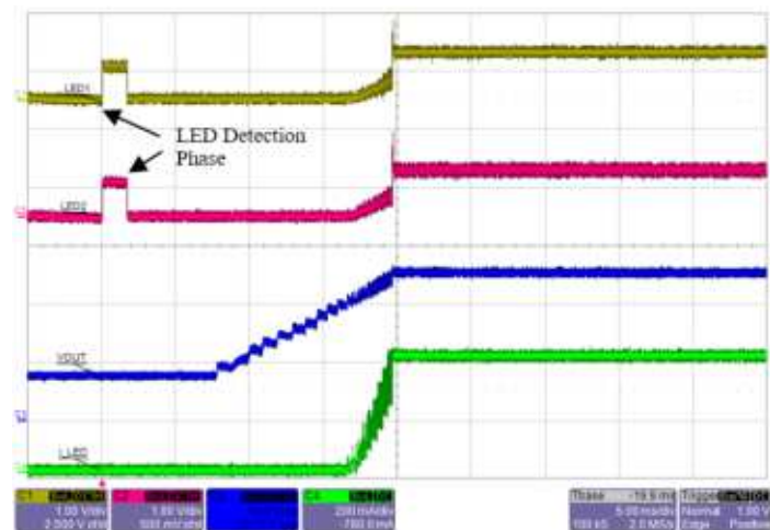
Figure 7: Normal startup showing all channels passed LED Detection phase. Total LED current = 100 mA × 4 (only LED1 and LED2 pin voltages are shown).
