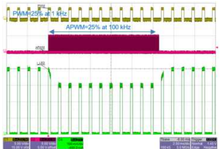
Figure 32: PWM = 25\% at 1\text{ kHz} . Peak LED current drops from 400\text{ mA} ( 4 \times 100\text{ mA/ch} ) to 300\text{ mA} when APWM of 25\% duty cycle is applied
