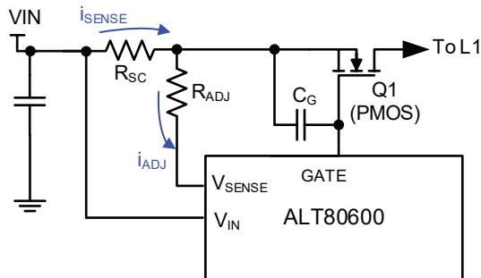
Figure 45: Optional input disconnect switch using a PMOSFET
