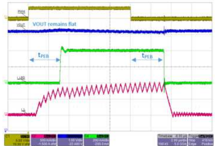
Figure 24: ALT80600 PWM dimming operation with PEB delay set to 3 \mu s. Note that V_{OUT} ripple is reduced to ~0.2 V.
