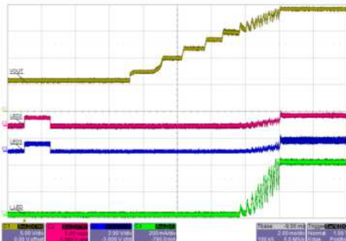
Figure 39: Normal startup sequence showing voltage at LED2 and LED3 pins. V_{IN} = 6 V, output = 6 × WLED in series, current = 4 × 100 mA
