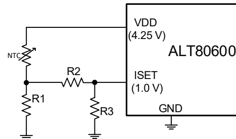
Figure 35: Thermal foldback of LED current using NTC thermistor
