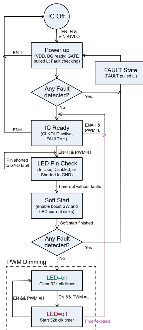
Figure 11: Startup Flow Chart
