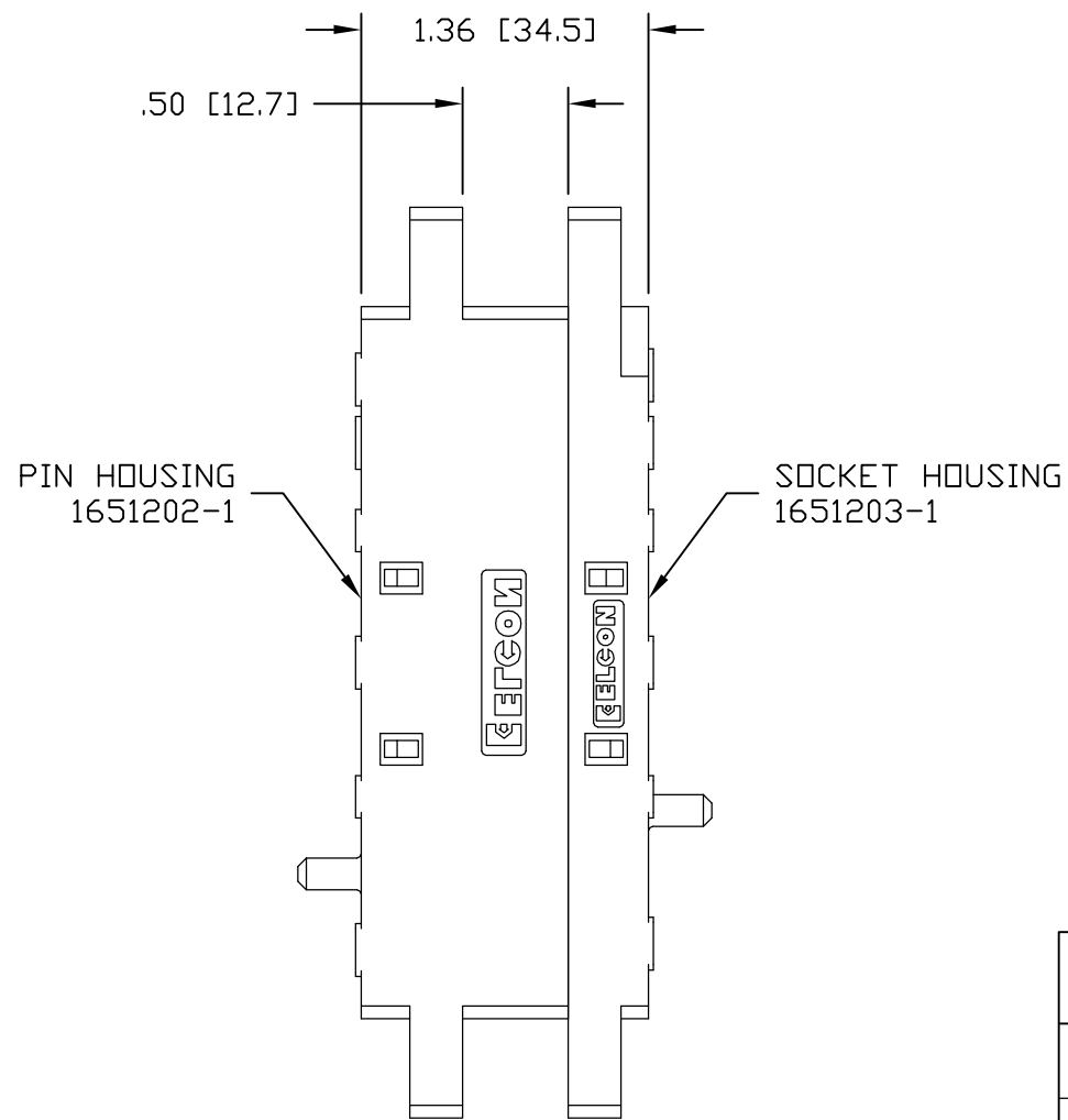
MATED CONDITION
