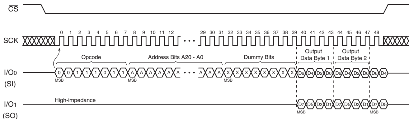
Figure 49. Dual-Output Read Array (Opcode 3Bh)
