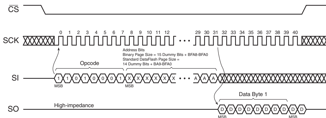
Figure 52. Buffer Read - Low Frequency (Opcode D1h or D3h)
