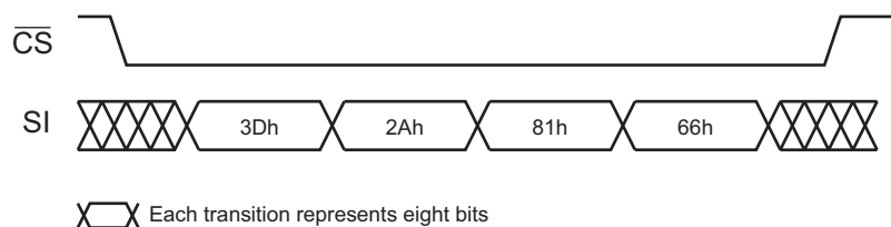
Figure 17. Quad Enable
