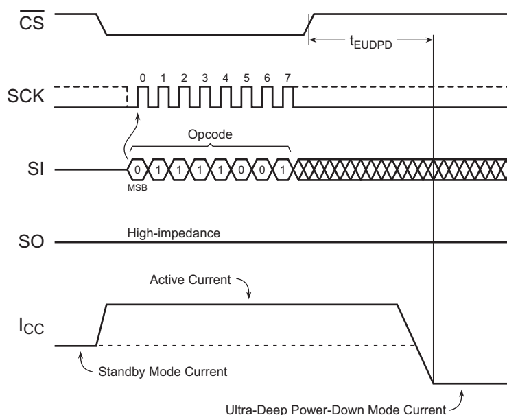
Figure 21. Ultra-Deep Power-Down
