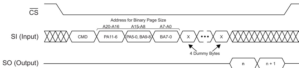
Figure 42. Main Memory Page Read
