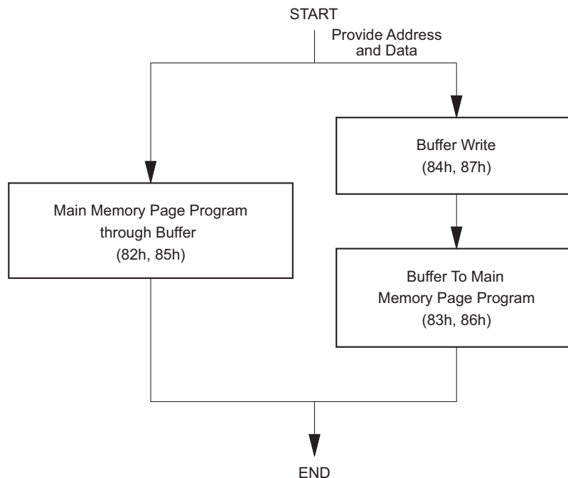
Figure 59. Algorithm for Programming or Re-Programming of the Entire Array Sequentially
