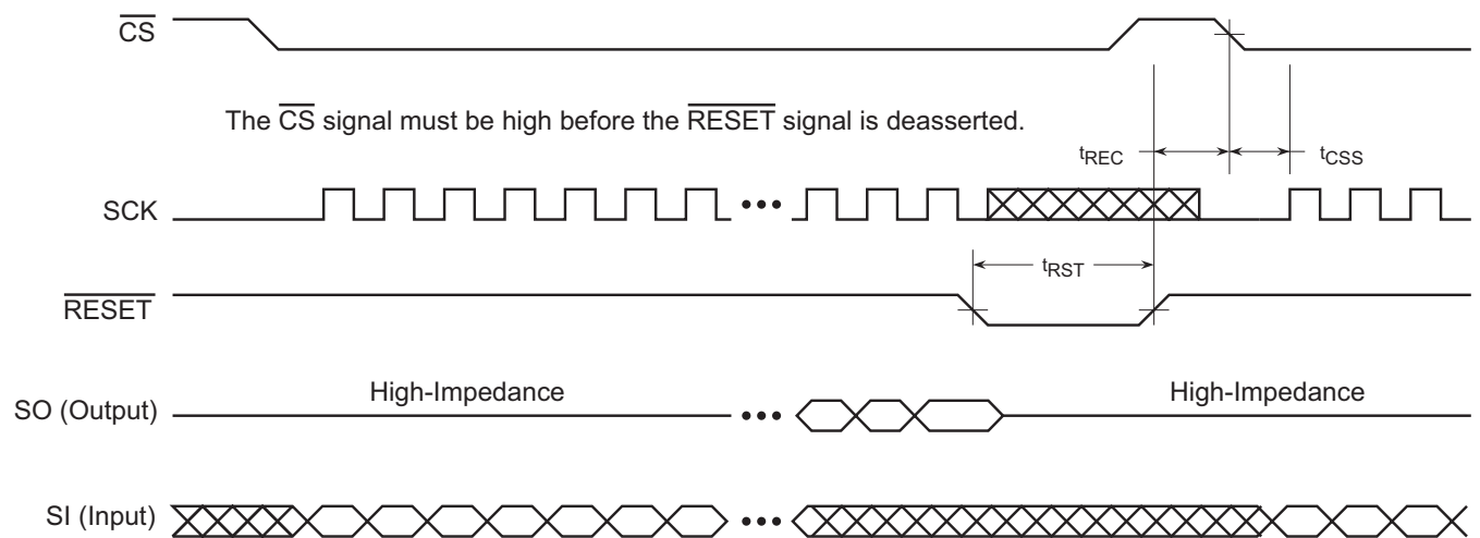
Figure 58. Reset Timing
