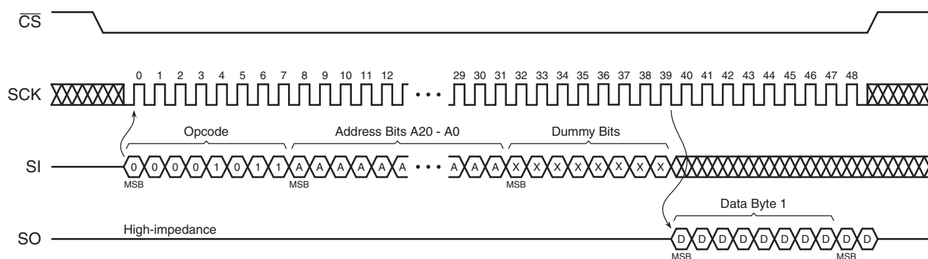
Figure 46. Continuous Array Read (Opcode 0Bh)
