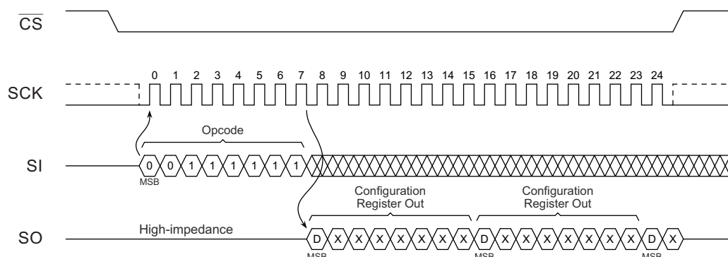
Figure 16. Read Configuration Register
