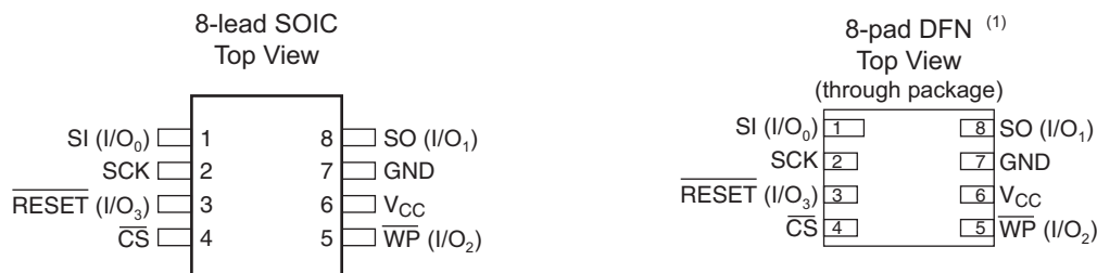
Figure 1. Pinouts
