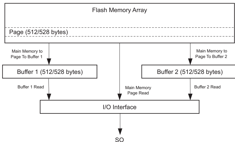
Figure 41. Block Diagram - Read
