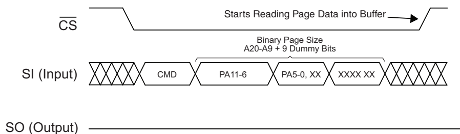
Figure 43. Main Memory Page to Buffer Transfer
