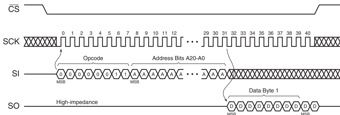
Figure 47. Continuous Array Read (Opcode 01h or 03h)
