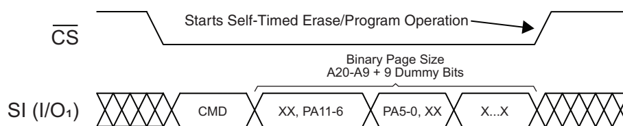
Figure 40. Buffer to main Memory Page Program
