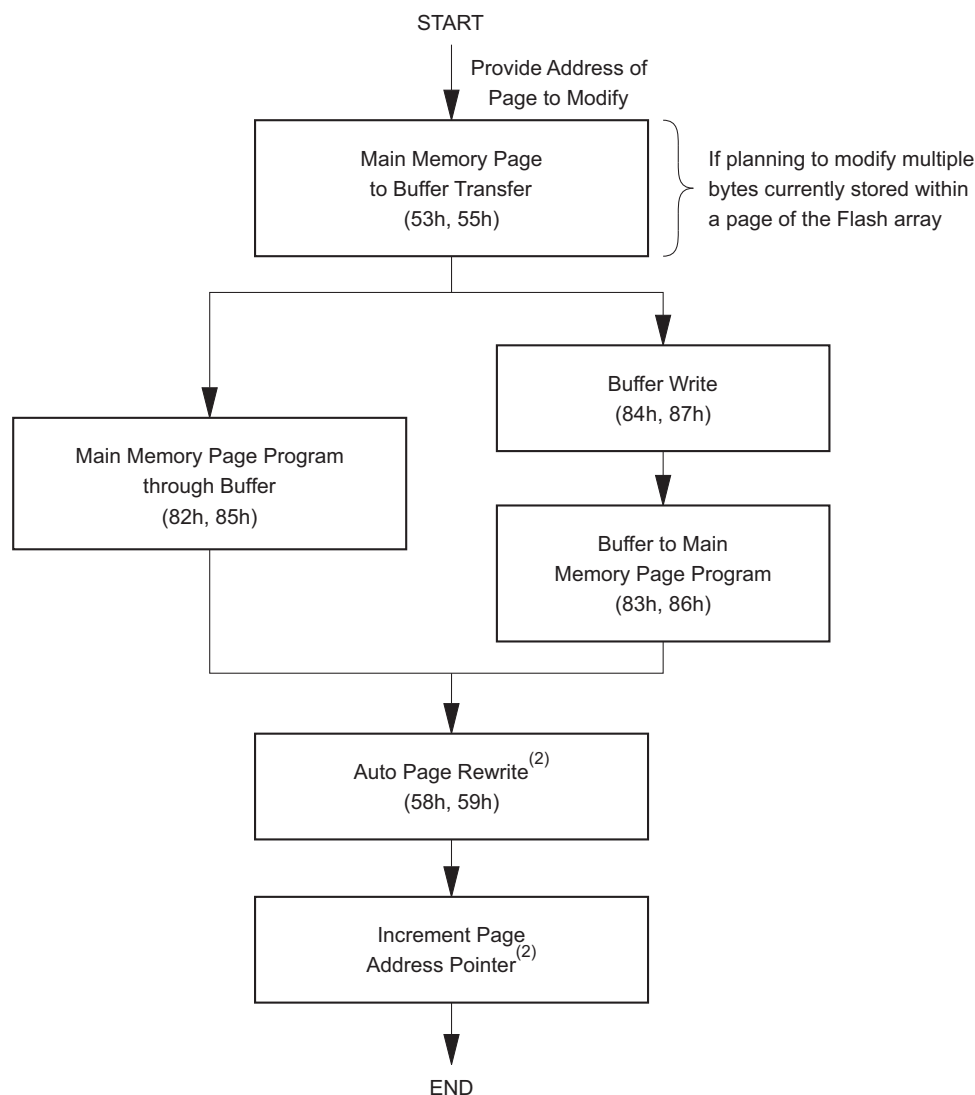
Figure 60. Algorithm for Programming or Re-Programming of the Entire Array Randomly
