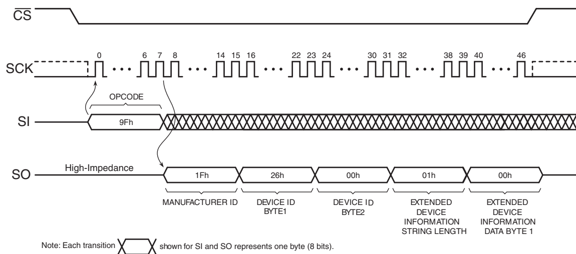
Figure 24. Read Manufacturer and Device ID
