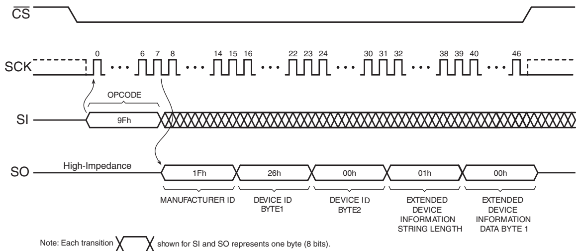
Figure 57. Manufacturer and Device Read (Opcode 9Fh)
