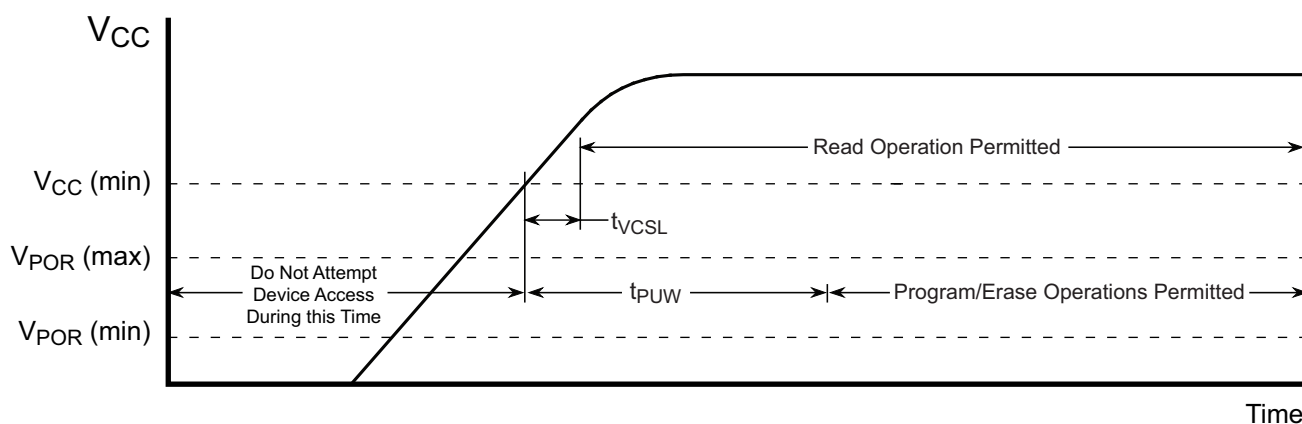
Figure 26. Power-Up Timing
