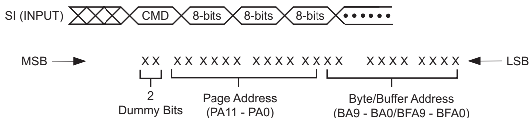
Figure 31. Command Sequence for Read/Write Operations for Page Size 528 Bytes
