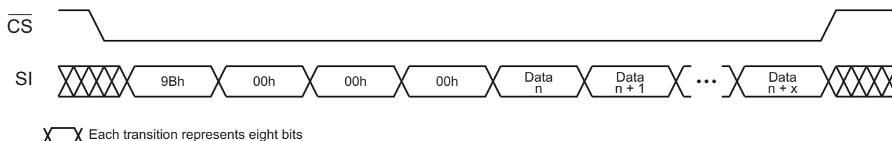
Figure 14. Figure 8-4. Program Security Register
