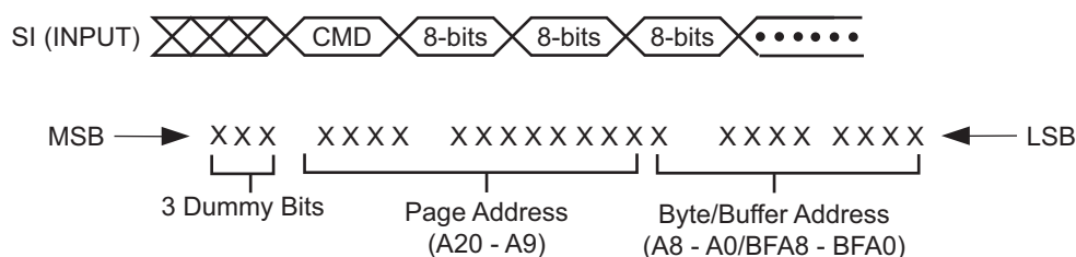
Figure 30. Command Sequence for Read/Write Operations for Page Size 512 Bytes
