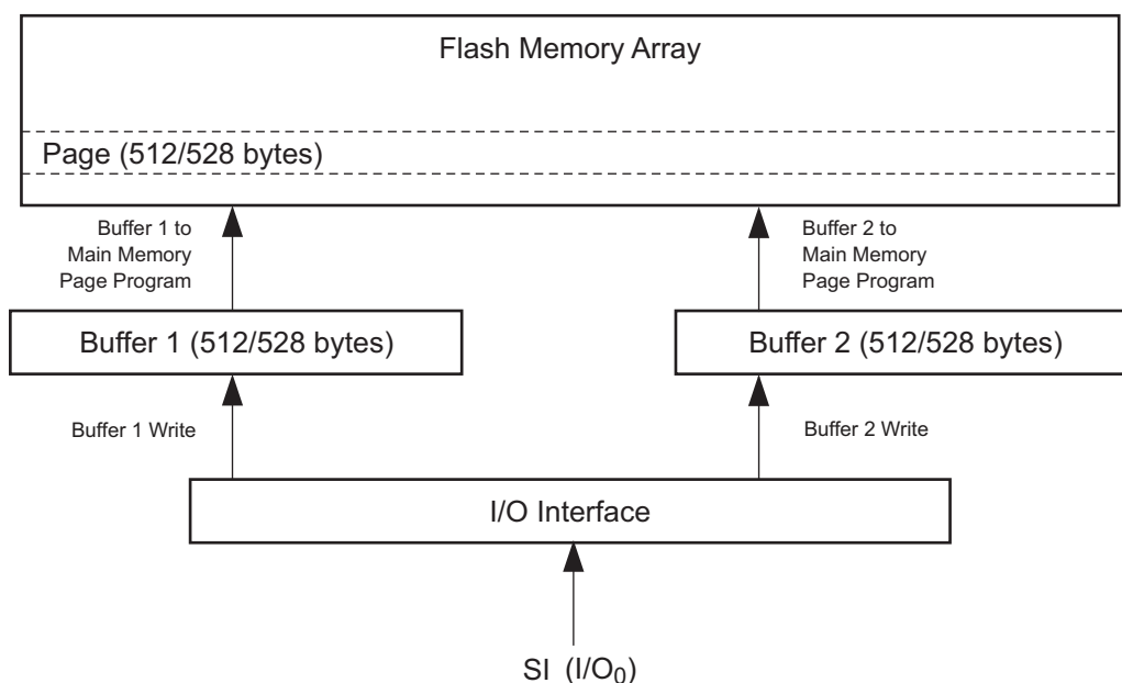
Figure 36. Block Diagram - Write
