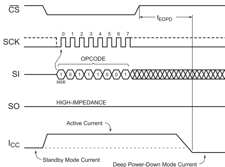
Figure 19. Deep Power-Down
