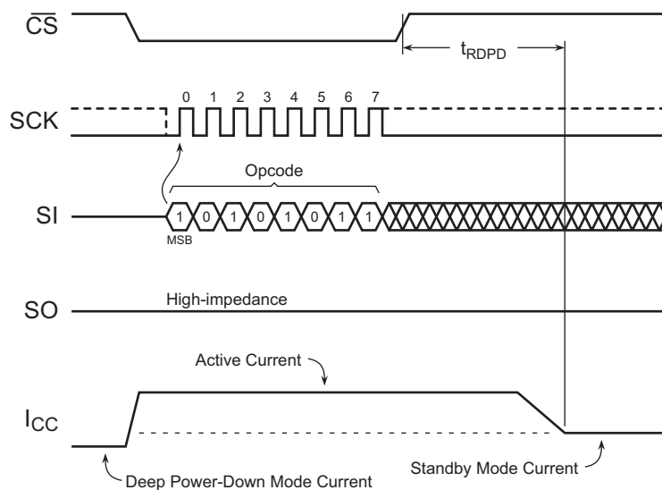
Figure 20. Resume from Deep Power-Down
