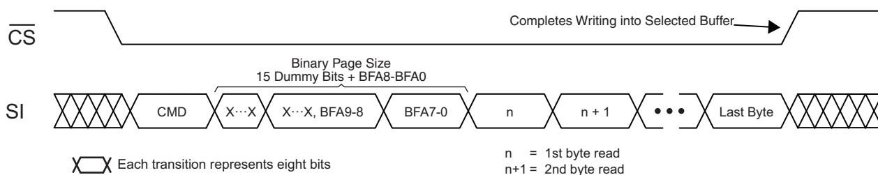
Figure 37. Buffer Write
