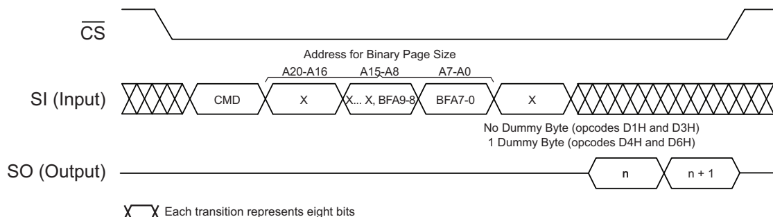
Figure 44. Buffer Read
