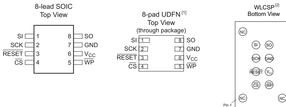
Figure 1. Pinouts
