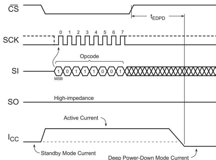
Figure 16. Deep Power-Down
