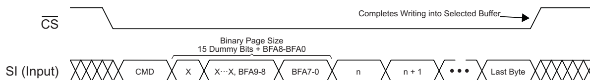
Figure 32. Buffer Write
