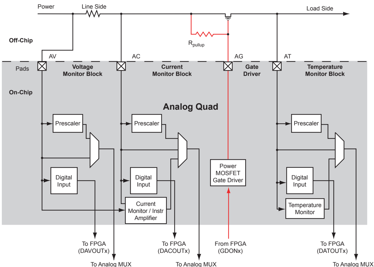
Figure 2-73 • Gate Driver
