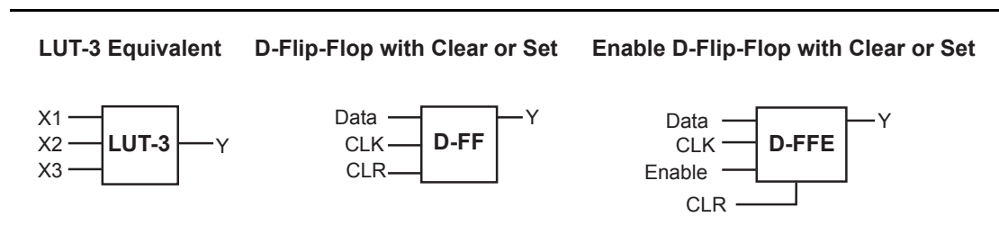
Figure 1-2 • VersaTile Configurations
