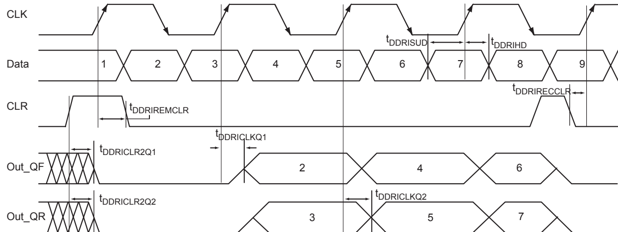
Figure 2-141 • Input DDR Timing Diagram
