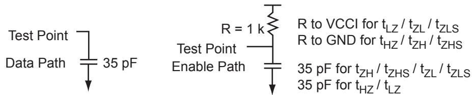
Figure 2-120 • AC Loading
