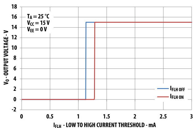
Figure 11 I_{FLH} Hysteresis
