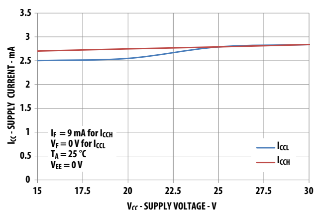
Figure 10 I_{CC} vs. V_{CC}
