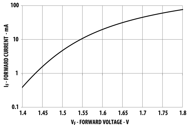
Figure 18 Input Current vs. Forward Voltage
