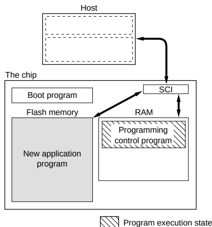
Figure 21.4 Boot Mode
