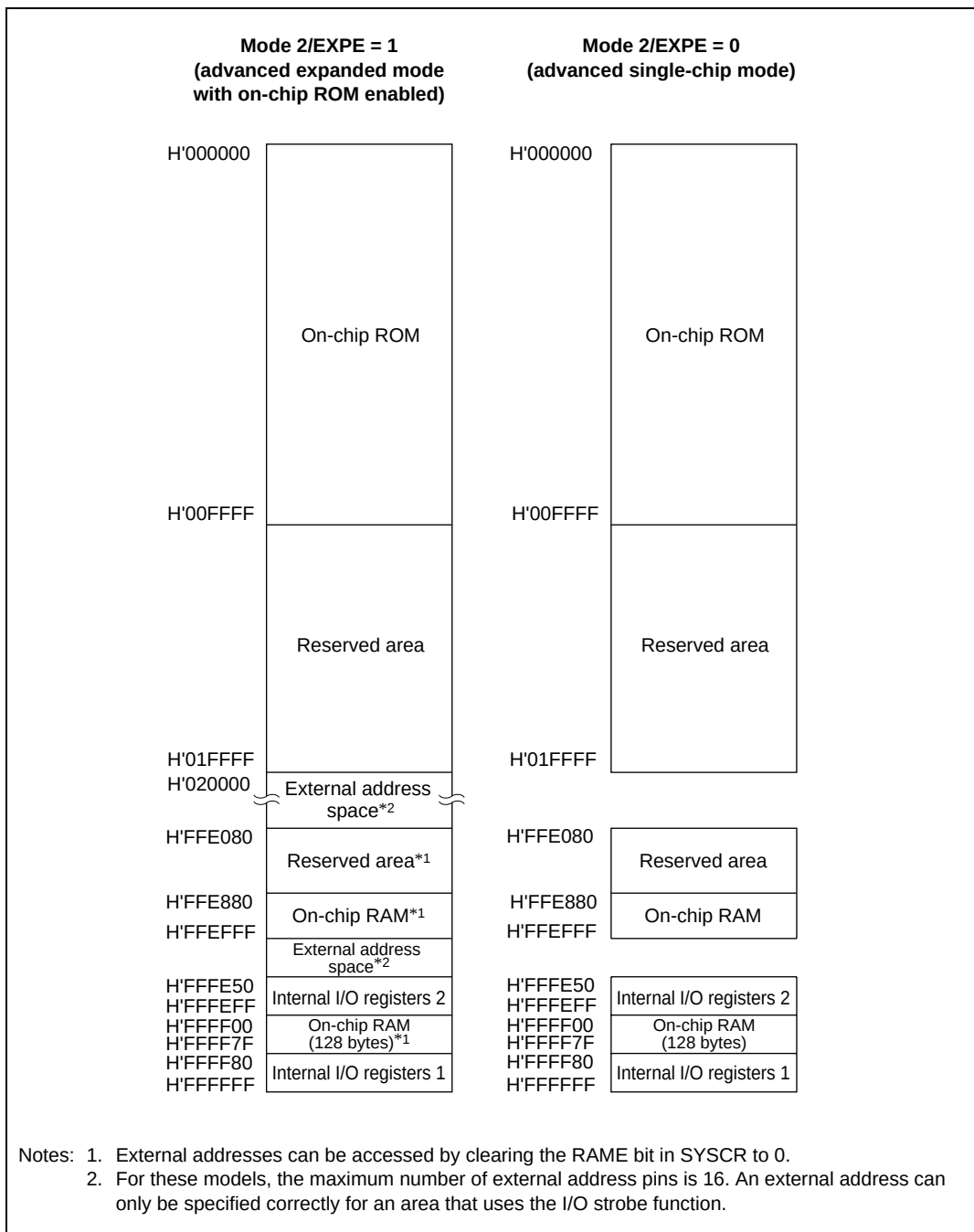
Figure 3.4 H8S/2137 and H8S/2132 Memory Map in Each Operating Mode (cont)
