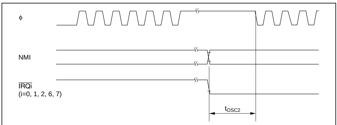
Figure 25.7 Oscillation Settling Timing (Exiting Software Standby Mode)
