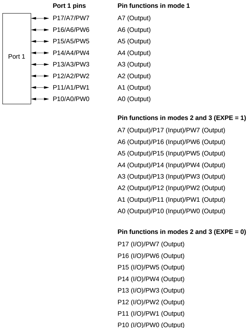
Figure 8.1 Port 1 Pin Functions
