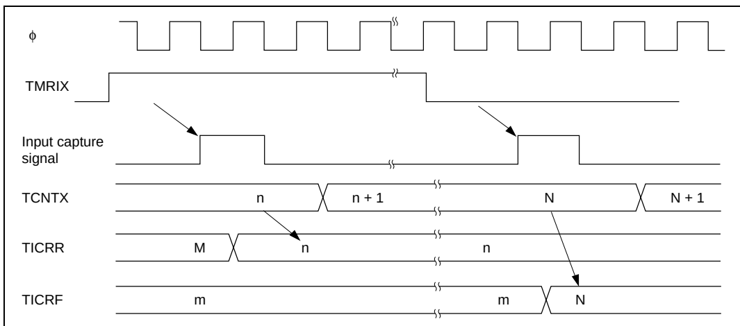
Figure 12.9 Timing of Input Capture Operation
