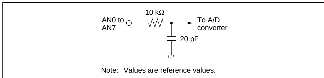
Figure 19.8 Analog Input Pin Equivalent Circuit
