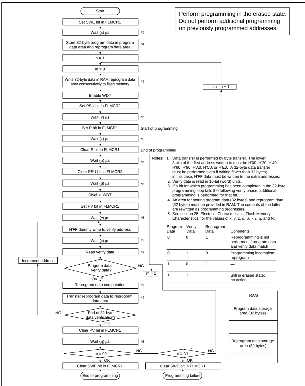
Figure 21.12 Program/Program-Verify Flowchart
