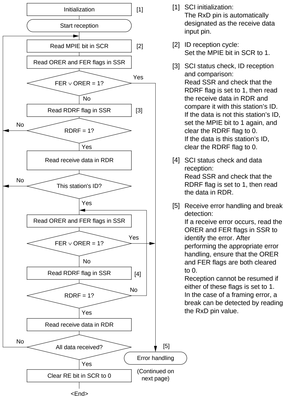
Figure 15.12 Sample Multiprocessor Serial Reception Flowchart
