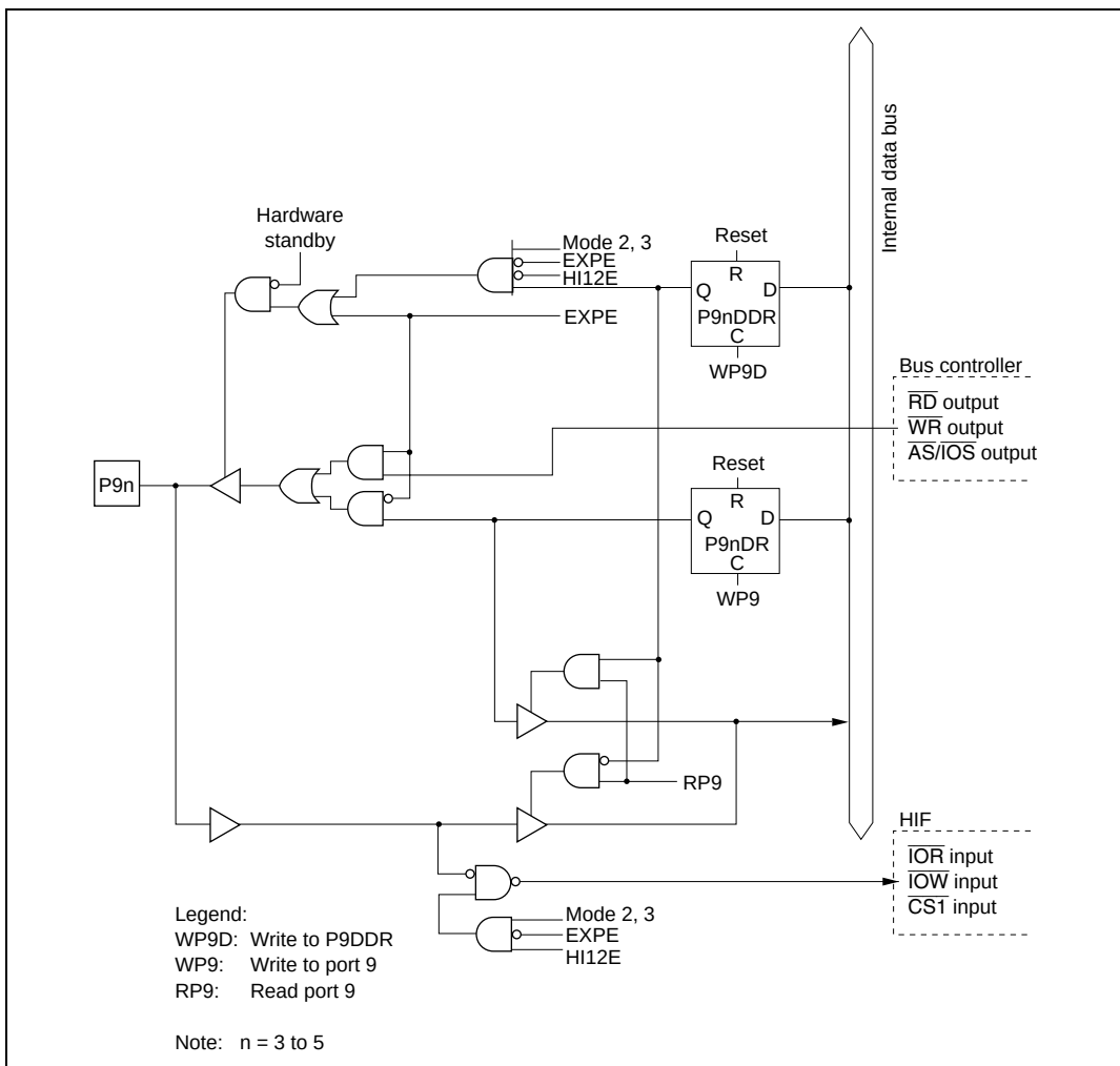
Figure C.31 Port 9 Block Diagram (Pins P93 to P95)
