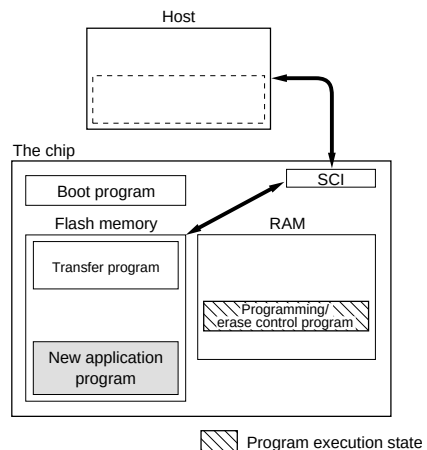
Figure 21.5 User Program Mode (Example)
