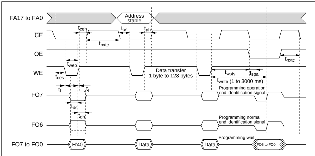
Figure 22.20 Auto-Program Mode Timing Waveforms
