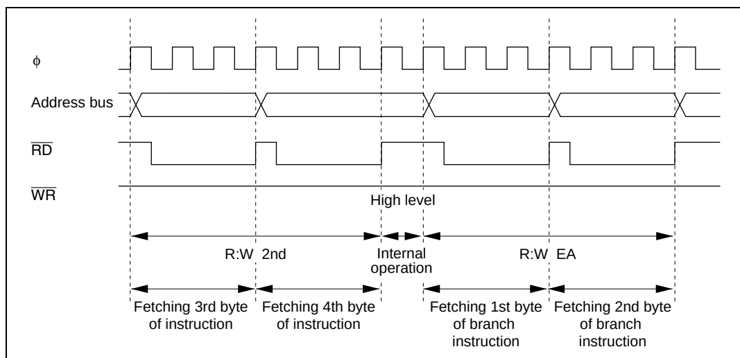
Figure A.1 Address Bus, \overline{RD} and \overline{WR} Timing (8-Bit Bus, Three-State Access, No Wait States)
