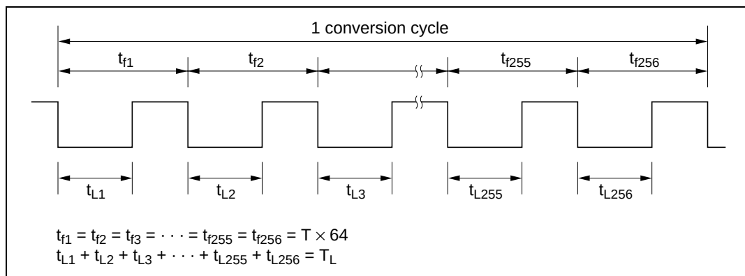
Figure 10.4 (1) Output Waveform
