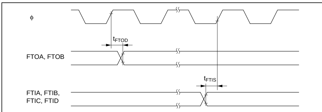
Figure 25.16 FRT Input/Output Timing
