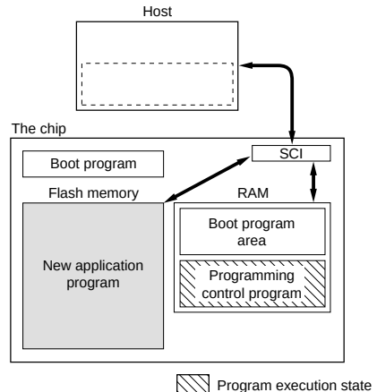
Figure 22.4 Boot Mode
