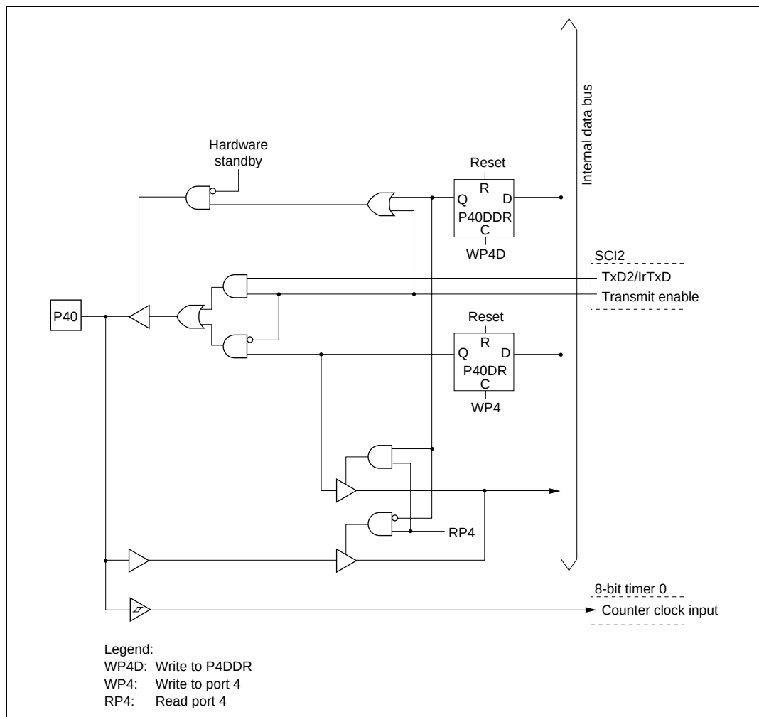
Figure C.6 Port 4 Block Diagram (Pin P40)
