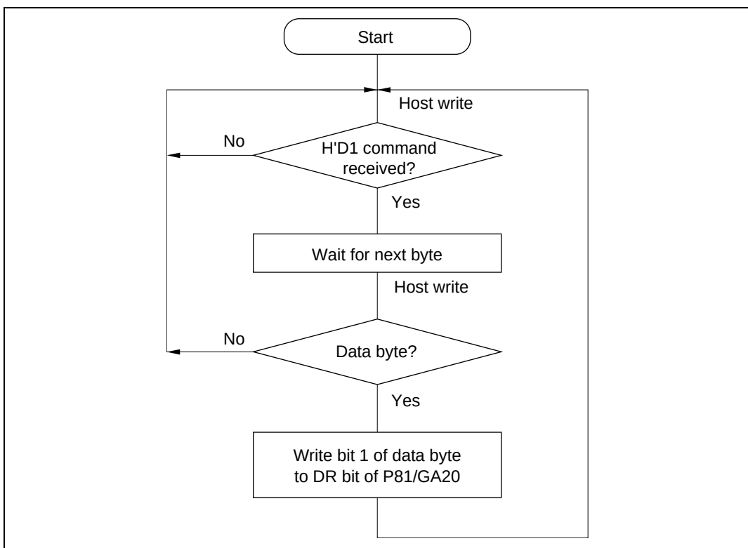
Figure 17.2 GA20 Output
