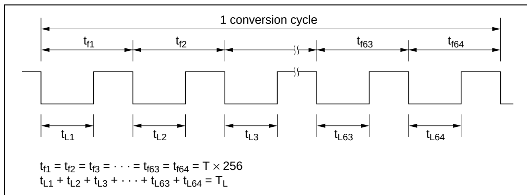
Figure 10.4 (2) Output Waveform
