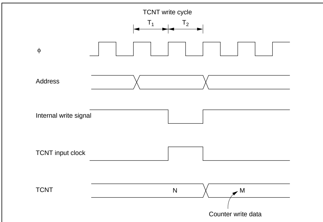
Figure 14.6 Contention between TCNT Write and Increment
