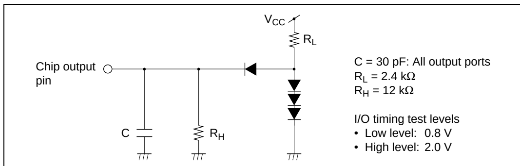
Figure 25.4 Output Load Circuit
