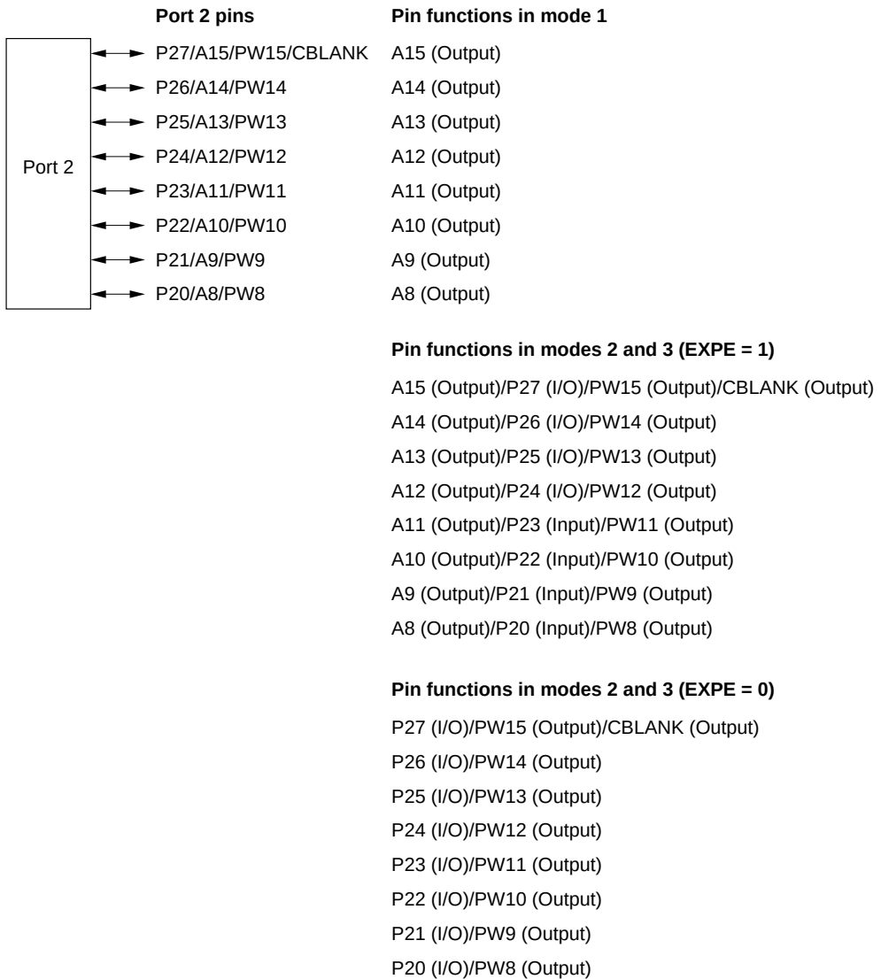
Figure 8.5 Port 2 Pin Functions
