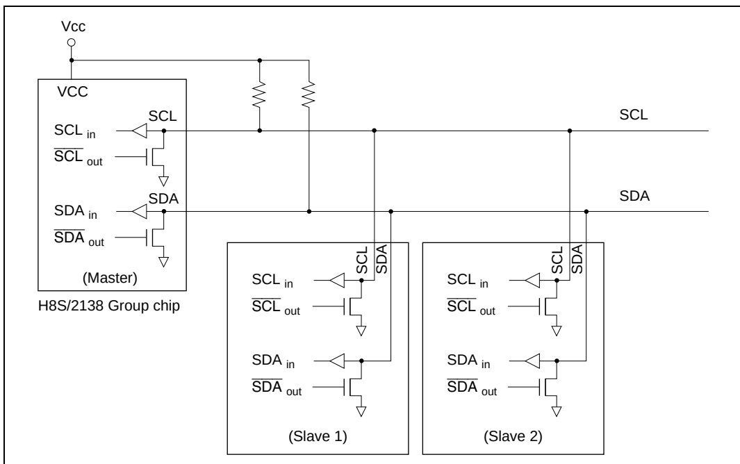
Figure 16.2 I 2 C Bus Interface Connections (Example: H8S/2138 Group Chip as Master)
