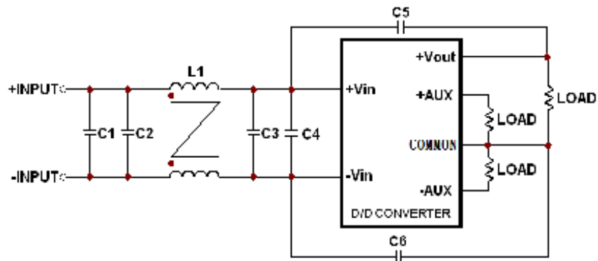
Suggested Schematic for EN55022 Conducted Emission Class B Limits
