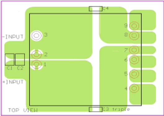
Recommended Layout with Input Filter
