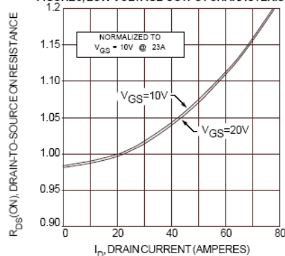
FIGURE 5, R_{DS(ON)} vs DRAIN CURRENT
