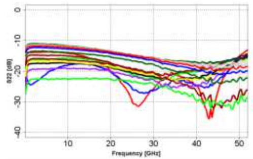
MMS004AA S22
