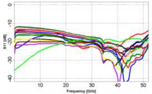
MMS004AA S11
