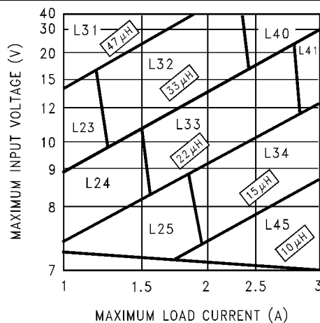
Figure 7-3. LM2670 – 5 V
