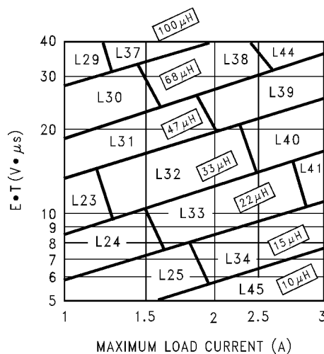
Figure 7-5. LM2670 – Adjustable
