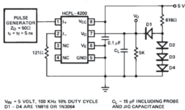
Figure 8. Test Circuit for t_{PHL} , t_{PLH} , t_f , and t_r
