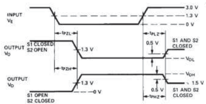
Figure 13. Waveforms for t_{PZH} , t_{PLZ} , t_{PHZ} , and t_{PLZ} .
