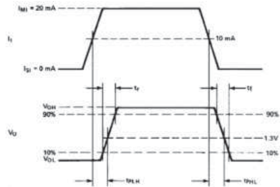
Figure 9. Waveforms for t_{PHL} , t_{PLH} , t_f , and t_r .
