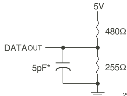
Figure 2. AC Test Load (for tOLZ, tOLZ, tCHZ, tOHZ, tOW, and tWHZ)
