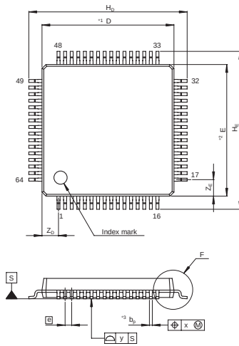
Figure E.2 Package Dimensions (FP-64E)
