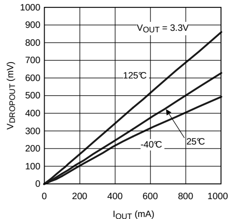
Figure 22. Dropout Voltage vs I_{OUT}
