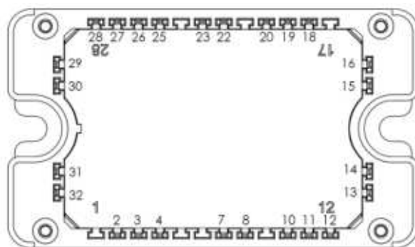
Figure 2 • MSCSM120SKM11CT3AG Pinout Location
