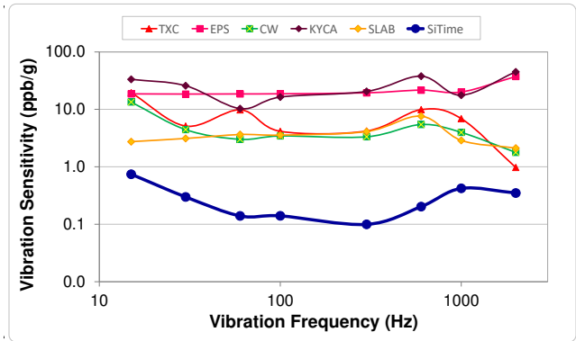
Figure 5. Vibration Robustness [5]
