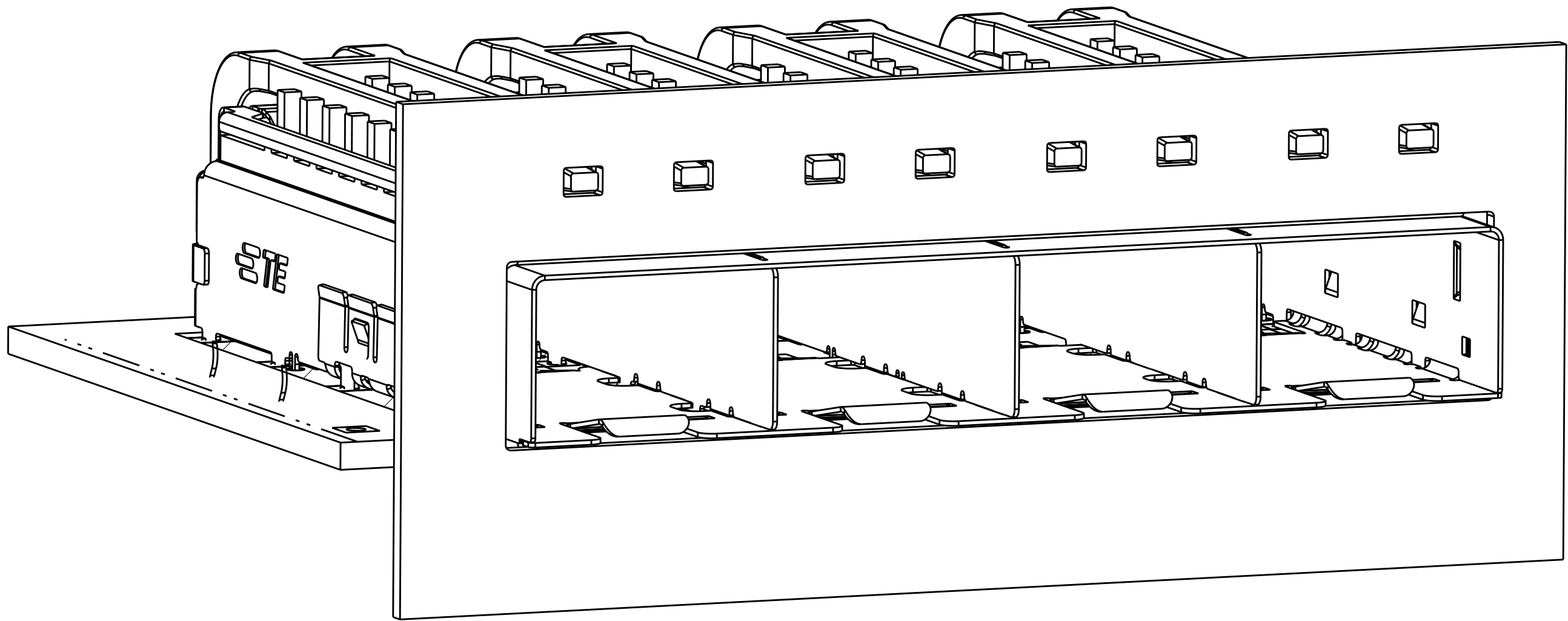
2198243-5 MOUNTED ON PCB SHOWN THRU RECOMMENDED BEZEL SCALE 4:1
