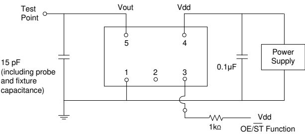
Figure 2. Test Circuit [6]
