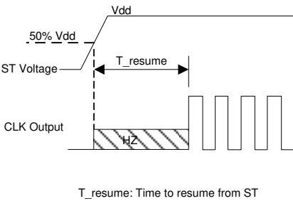
Figure 6. Standby Resume Timing (ST Mode Only)
