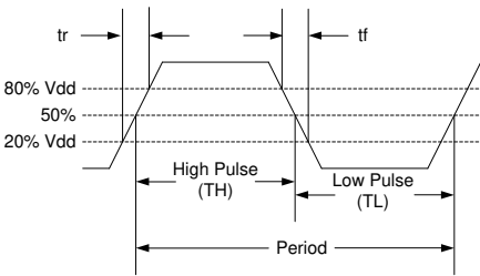
Figure 3. Output Waveform [6]
