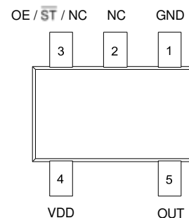
Figure 1. Pin Assignments
