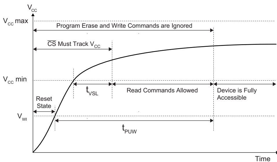
Figure 68. Power-Up Timing and Voltage Levels
