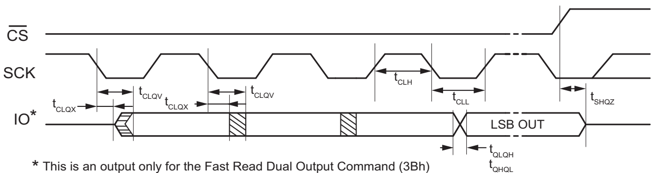
Figure 71. Output Timing
