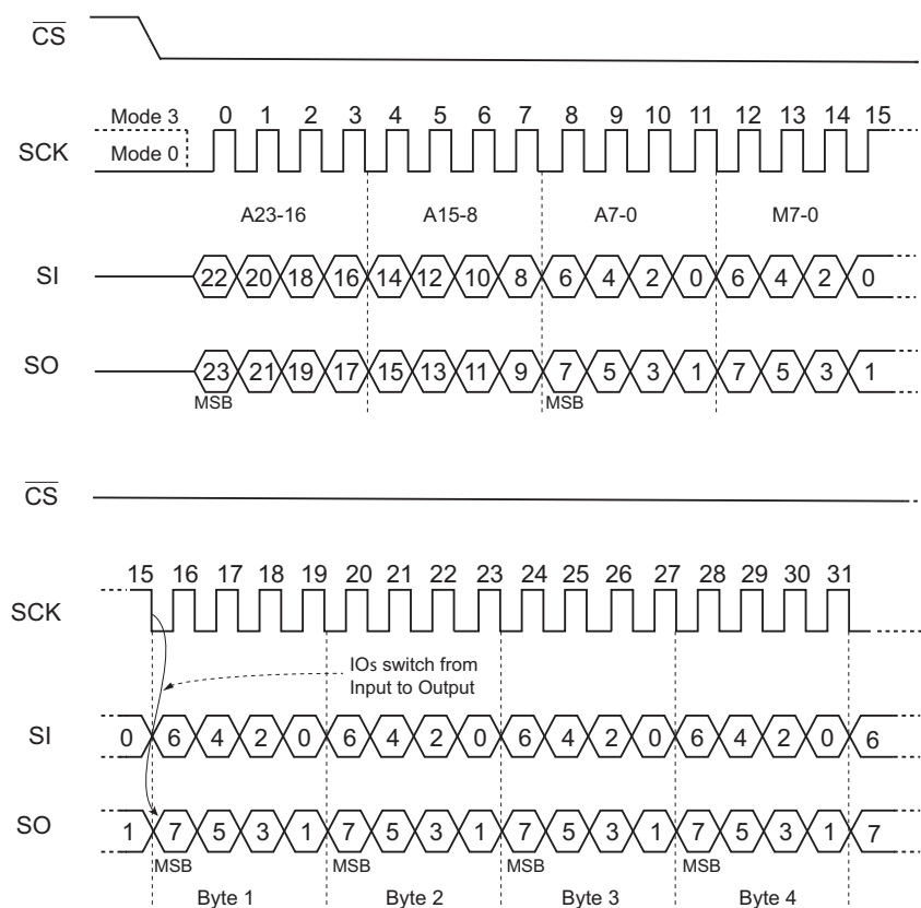
Figure 22. Fast Read Dual I/O Command (previous M7-0 = Axx)
