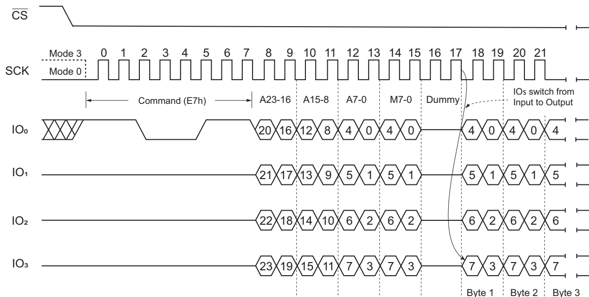
Figure 54. Word Read Quad I/O command (Initial command or previous set M7-0 ≠ Axx, SPI Mode)
