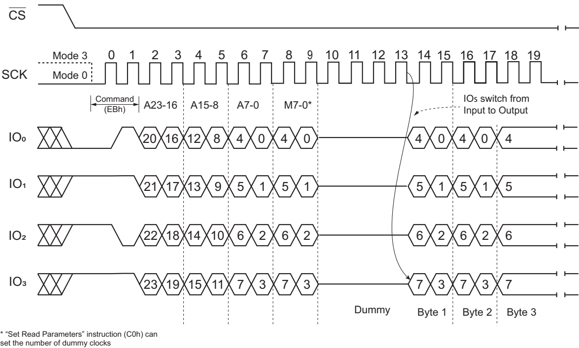
Figure 26. Fast Read Quad I/O Command (Initial command or previous M7-0 ≠ Axx, QPI mode, 133 MHz)
