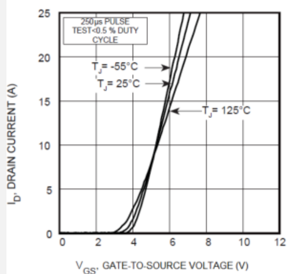
Figure 1-2. Transfer Characteristics
