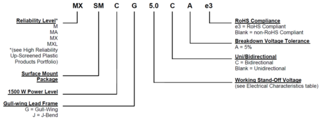
Figure 2-1. Part Nomenclature
