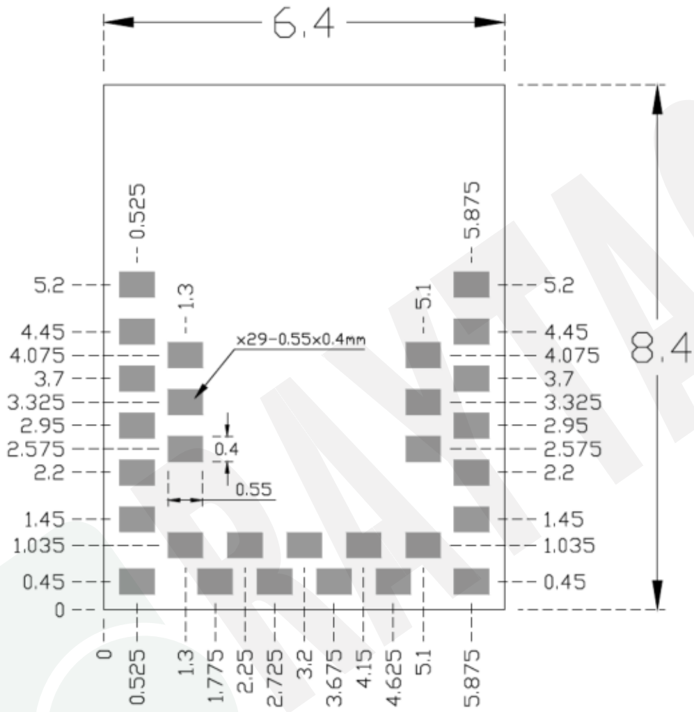
Top View (Unit: mm)
