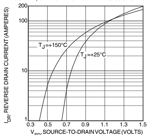
FIGURE 13, SOURCE-DRAIN DIODE FORWARD VOLTAGE
