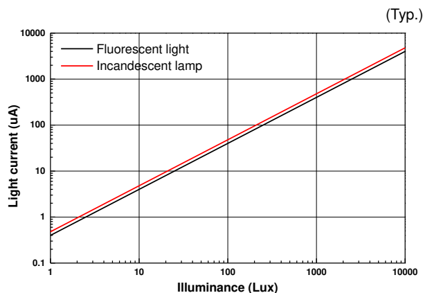
Fig 5. Light Output vs. Illuminance
