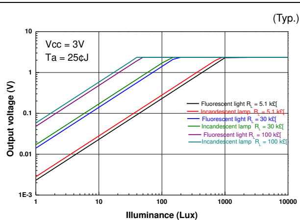
Fig 10. Output Voltage vs. Illuminance
