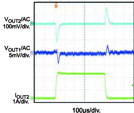
CH1 Steady State, CH2 Load Trasient
