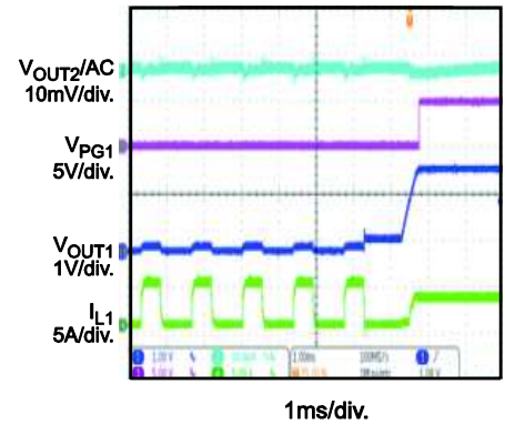
CH1 SCP Recovery, CH2 Steady State
