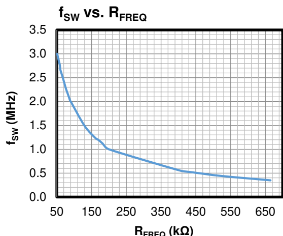
Figure 4: f_{SW} vs. R_{FREQ}
