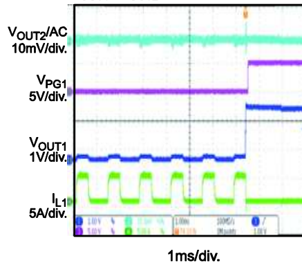
CH1 SCP Recovery, CH2 Steady State
