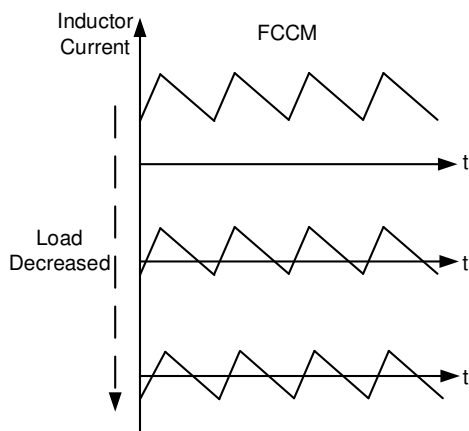
Figure 3: FCCM
