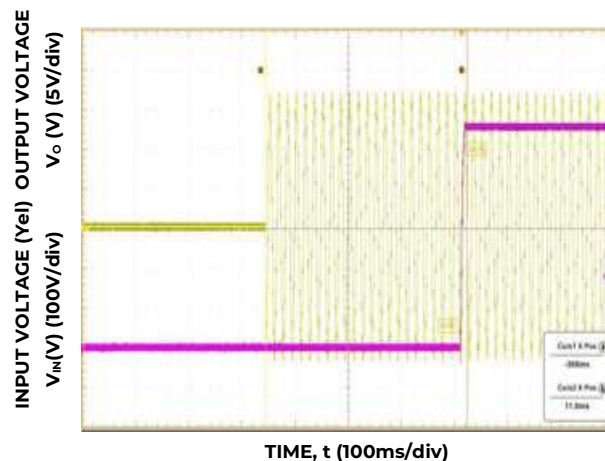
Figure 6. Typical Start-up ( V_{IN} = 230V_{AC} , Full load)
