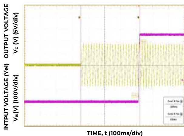
Figure 5. Typical Start-up ( V_{IN} = 115V_{AC} , Full Load).
