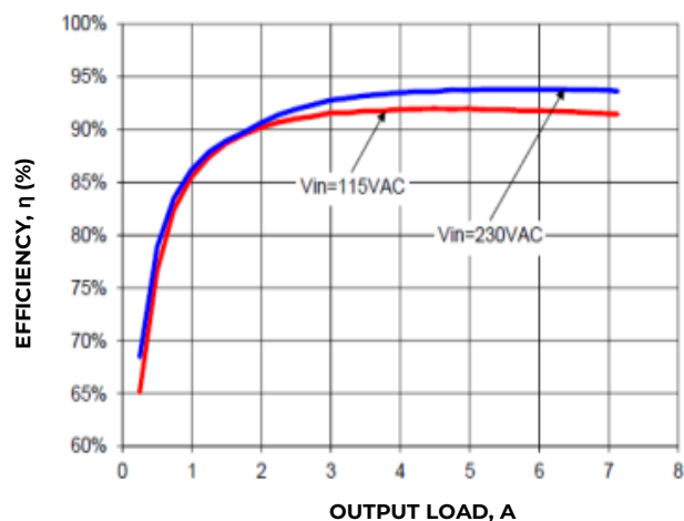
Figure 1. Power Supply Efficiency versus Output Current.
