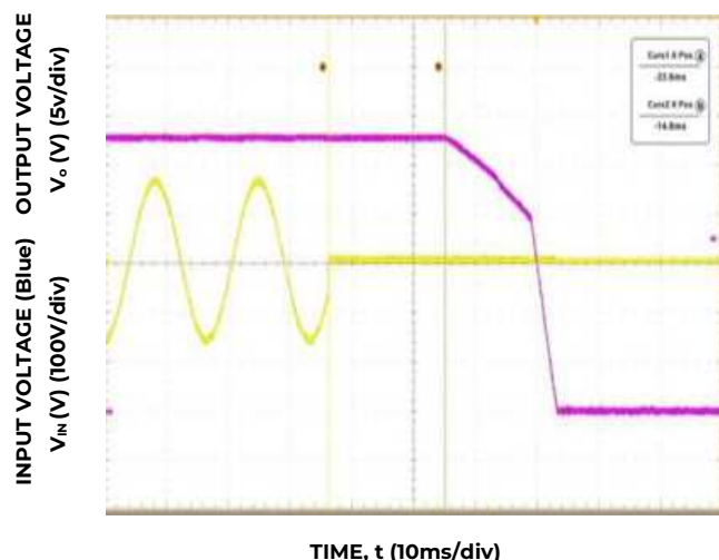
Figure 7. Typical Hold-up waveforms ( V_{IN} = 115V , 100% load).
