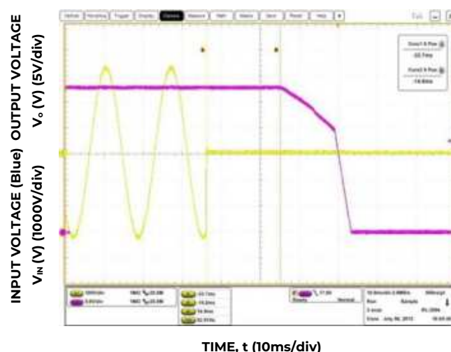
Figure 8. Typical Hold-up waveforms ( V_{IN} = 230V , 100% load).
