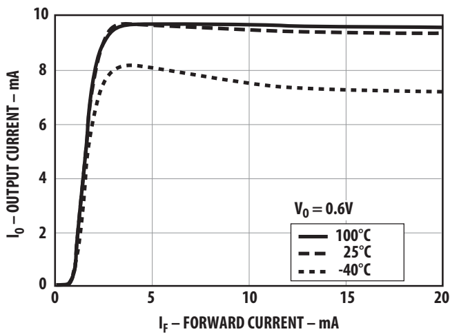
Figure 1 Typical Transfer Characteristics
