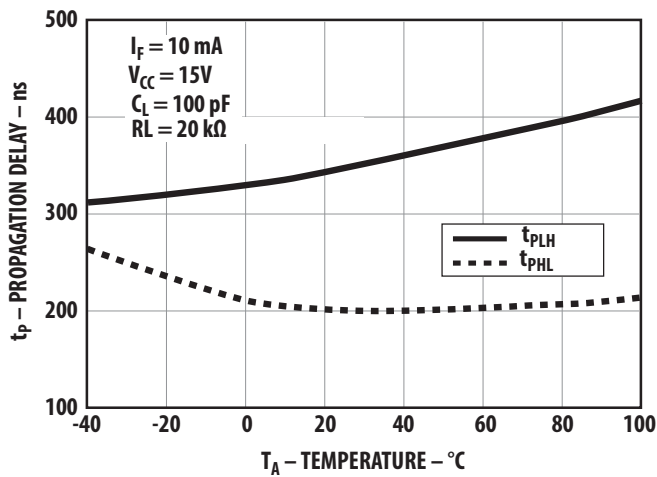
Figure 7 Propagation Delay with External 20\text{ k}\Omega R_L vs. Temp.
