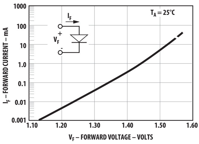
Figure 4 Input Current vs. Forward Voltage
