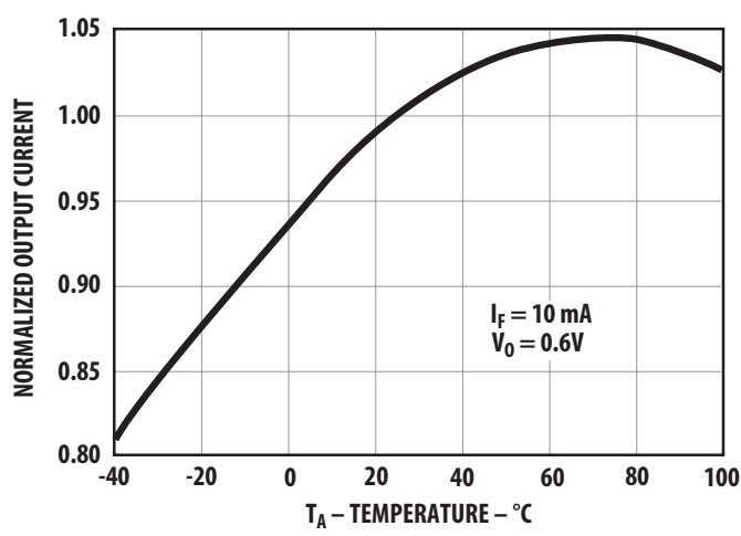
Figure 2 Normalized Output Current vs. Temperature
