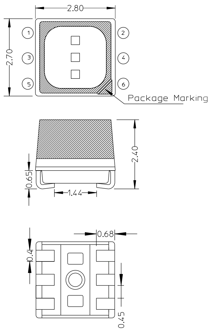
Figure 1: Package Drawing
