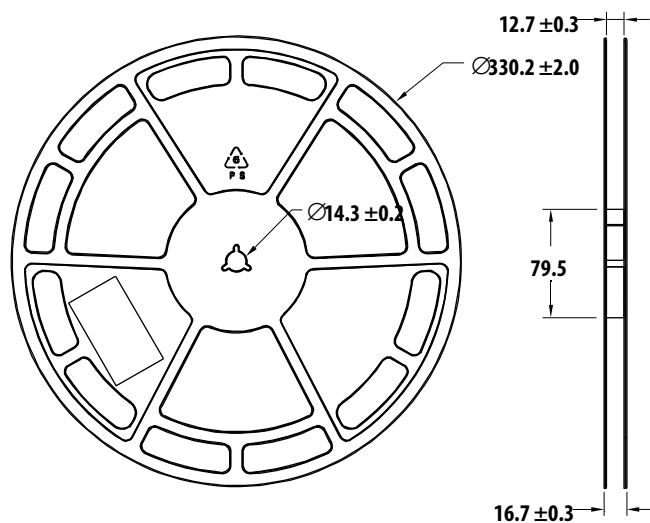
Figure 14: Reel Dimensions
