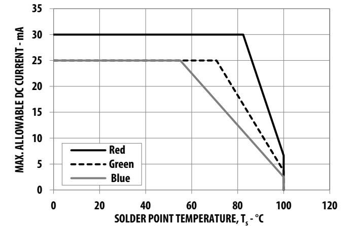
Figure 9: Maximum Forward Current vs. Solder Temperature for Red, Green, and Blue (1 chip and 3 chips on)
