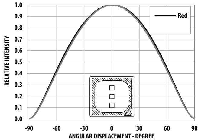
Figure 10: Radiation Pattern for x-Axis
