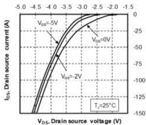
Figure 10 • Body Diode Characteristics, T_J = 25^\circ C
