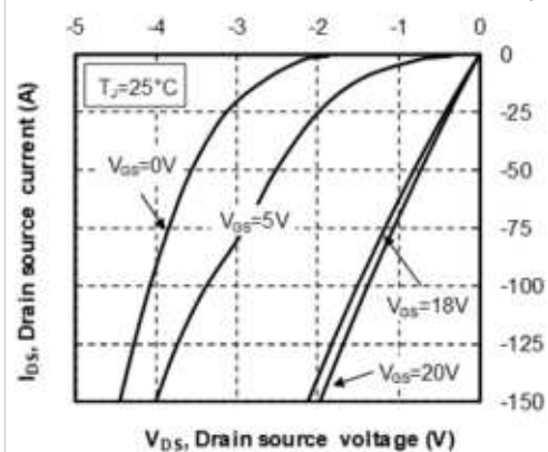
Figure 11 • 3 rd Quadrant Characteristics, T_J = 25^\circ C
