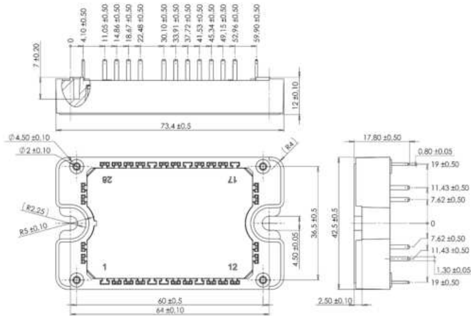
Figure 21 • Package Outline
