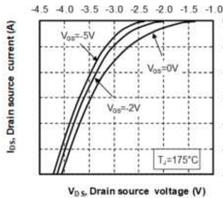
Figure 12 • Body Diode Characteristics, T_J = 175^\circ\text{C}
