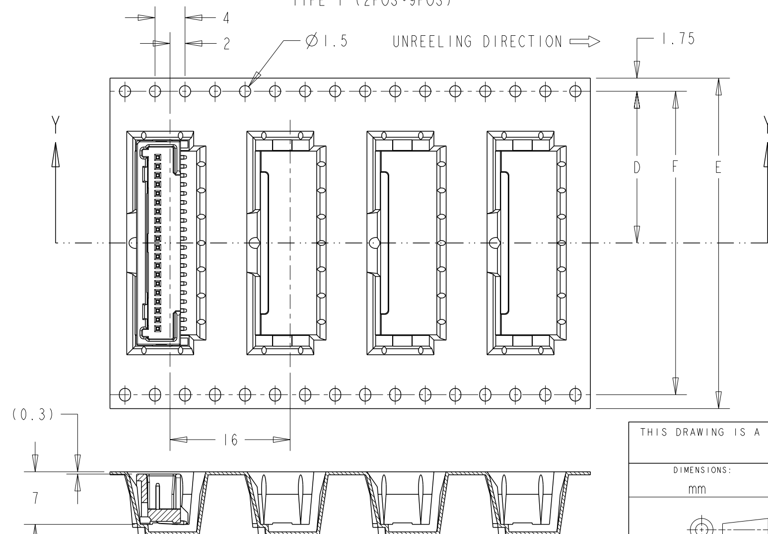
SECTION Y-Y TYPE 2 (10POS~25POS)
