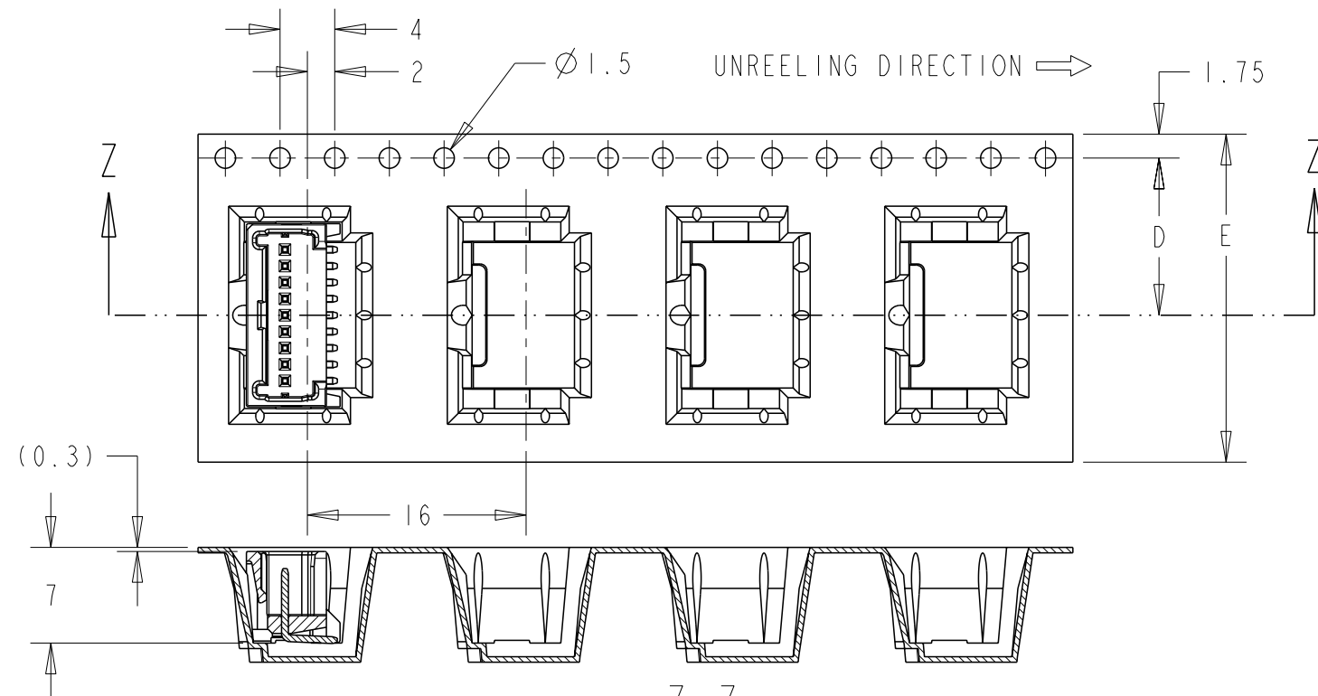
SECTION Z-Z TYPE I (2POS~9POS)
